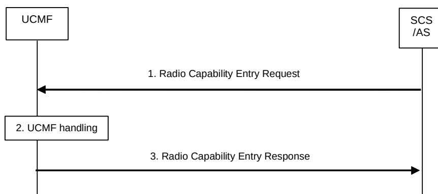
Figure 5.19.3-1: RACS information provisioning procedure via T9a
