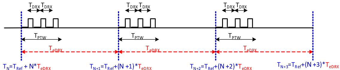
Figure 4.5.13.2-1 The usage of PTW and independence of the extended Idle mode DRX cycle from UE state
