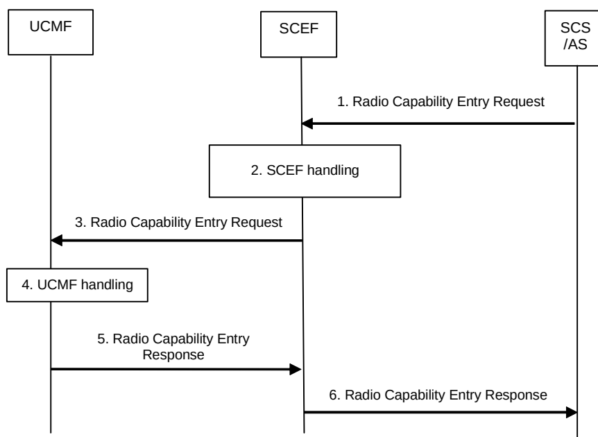
Figure 5.19.2-1: RACS information provisioning procedure via SCEF
