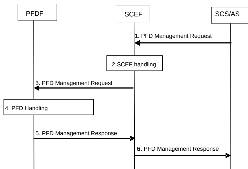
Figure 5.14.1-1: procedure for PFD management via SCEF
