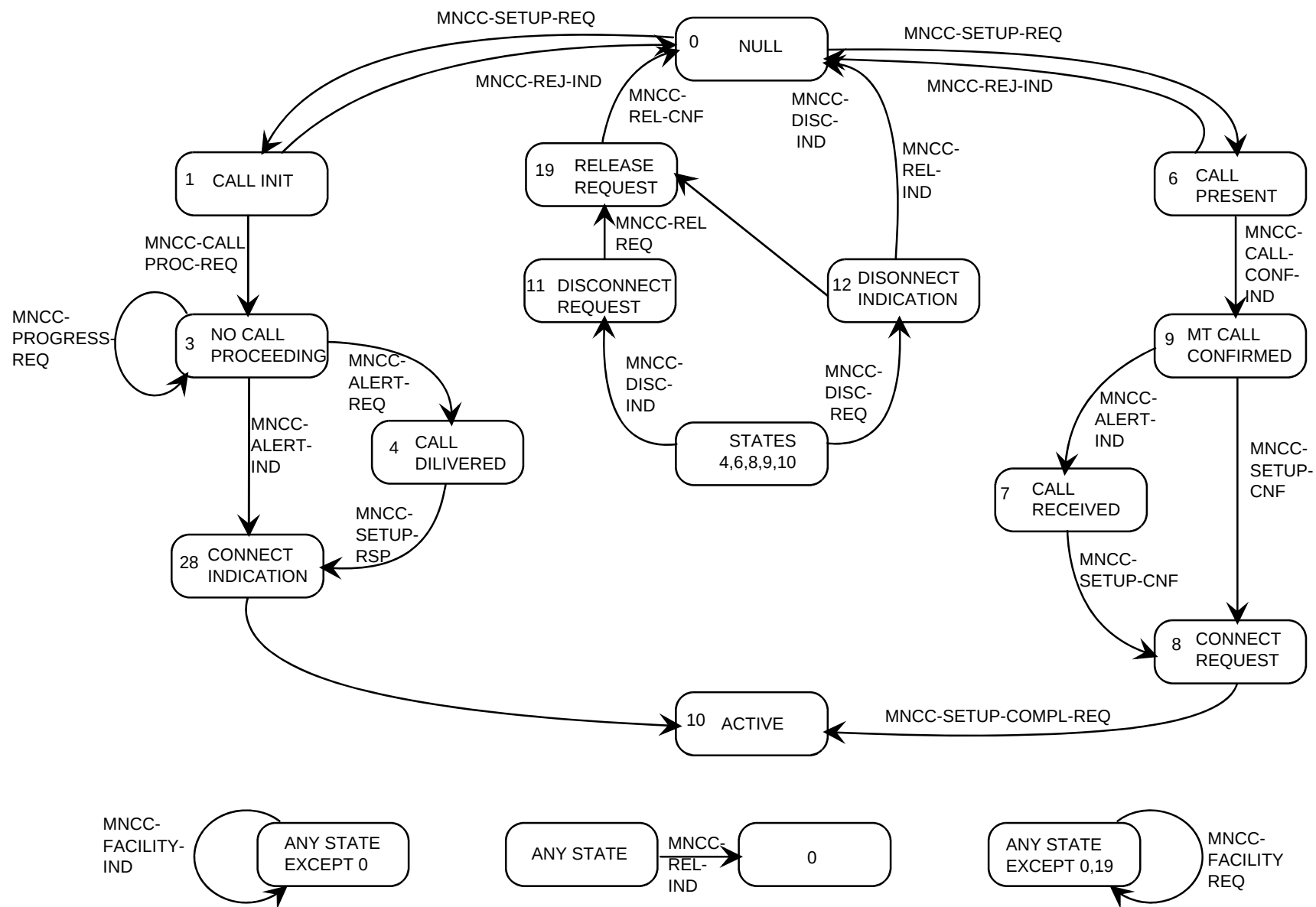
Figure 7.1: (page 1 of 2) Service graph of Call Control entity - Network side
