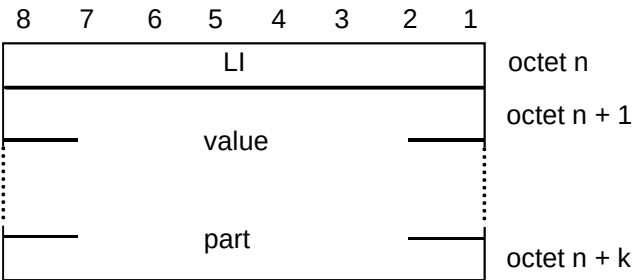
Figure 11.7: Type 4 IE of format LV (k = 0, 1, 2, ...)
