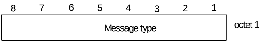
Figure 11.10d: Message type IE (protocol other than MM, CC, SS, GCC, BCC, LCS and AIoT NAS)
