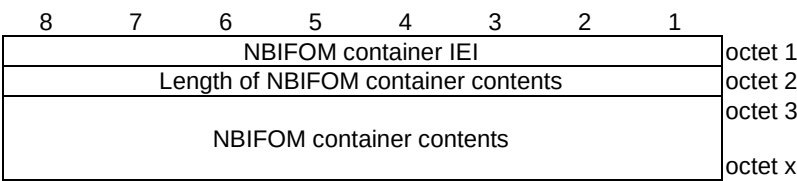
Figure 10.5.6.21-1/3GPP TS 24.008: NBIFOM container information element
