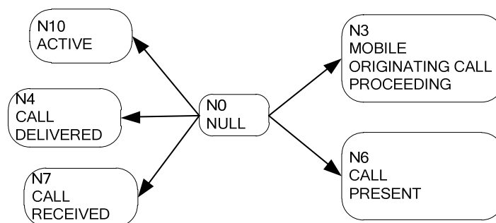
Figure 5.1b.2/3GPP TS 24.008: Overview call control protocol/Network side, extension for SRVCC from PS to CS or 5G-SRVCC handover from NG-RAN to UTRAN
