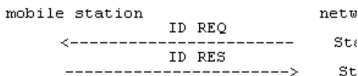
Figure 4.3/3GPP TS 24.008: Identification sequence
