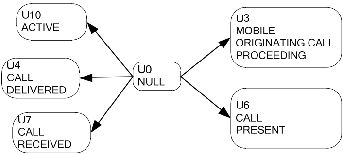
Figure 5.1a.2/3GPP TS 24.008: Overview call control protocol/MS side, extension for SRVCC from PS to CS or 5G-SRVCC handover from NG-RAN to UTRAN
