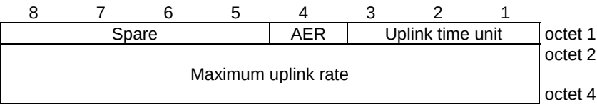
Figure 10.5.136A/3GPP TS 24.008: APN rate control parameters
