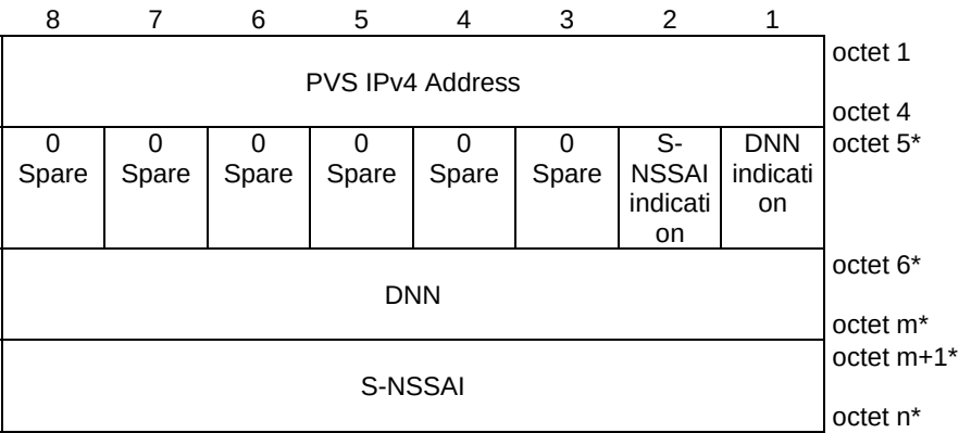
Figure 10.5.6.3.10-1/3GPP TS 24.008: PVS IPv4 Address
