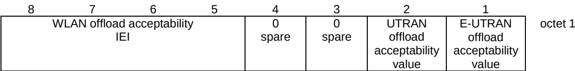
Figure 10.5.6.20-1/3GPP TS 24.008: WLAN offload acceptability information element
