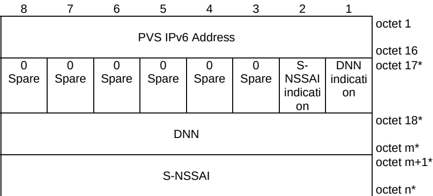
Figure 10.5.6.3.11-1/3GPP TS 24.008: PVS IPv6 Address
