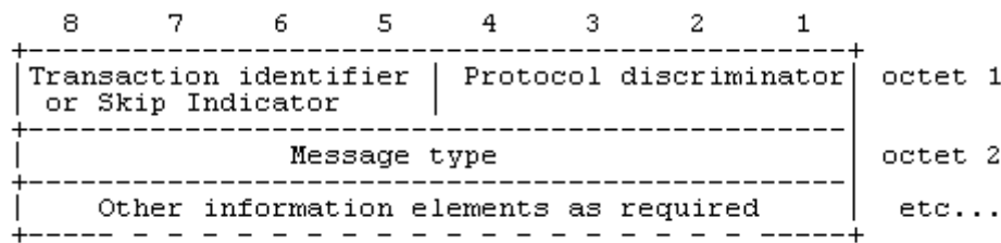
Figure 10.1/3GPP TS 24.008 General message organization example
