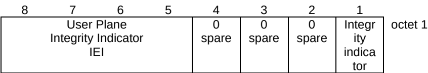
Figure 10.5.5.34-1/3GPP TS 24.008 User Plane integrity indicator information element
