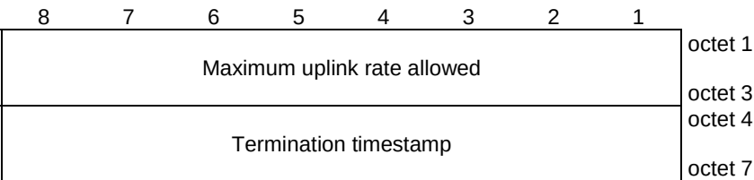
Figure 10.5.6.3.6-1/3GPP TS 24.008: Initial small data rate control parameters
