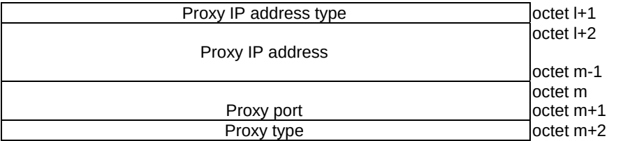
Figure 6.1.4.2-2: Proxy information
