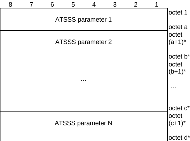
Figure 6.1.2-1: ATSSS container contents
