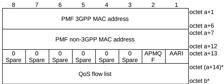
Figure 6.1.5.2-2: ATSSS parameter contents including one PMF MAC address information
