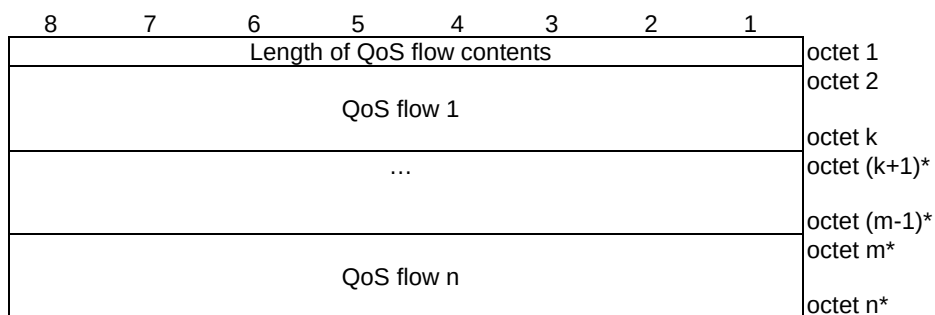
Figure 6.1.5.2-3: QoS flow list information element
