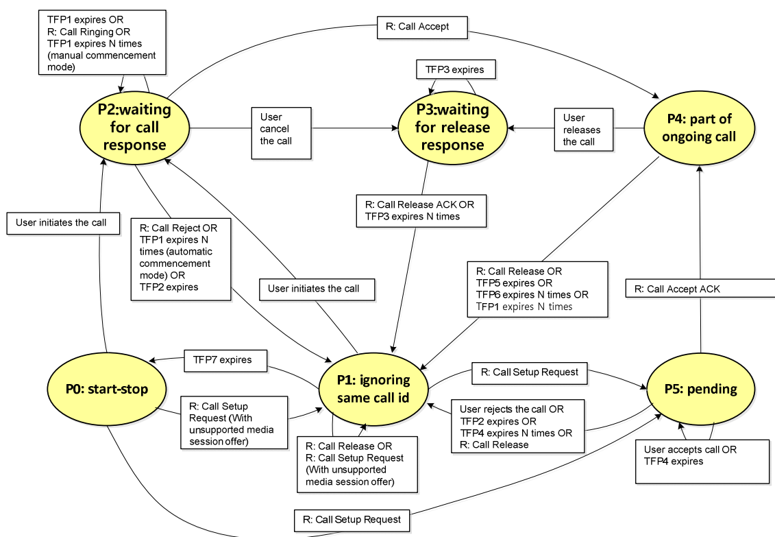
Figure 10.3.2.2-1: Private call control state machine
