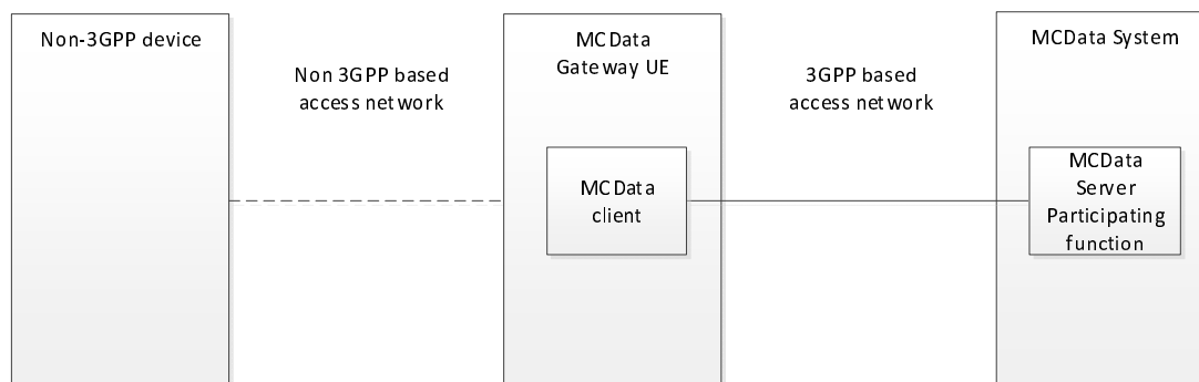
Figure 5.5.2-1: Relationship between non-3GPP device, MCDATA gateway UE and the MCDATA server with the MCDATA client located in the MCDATA gateway UE
