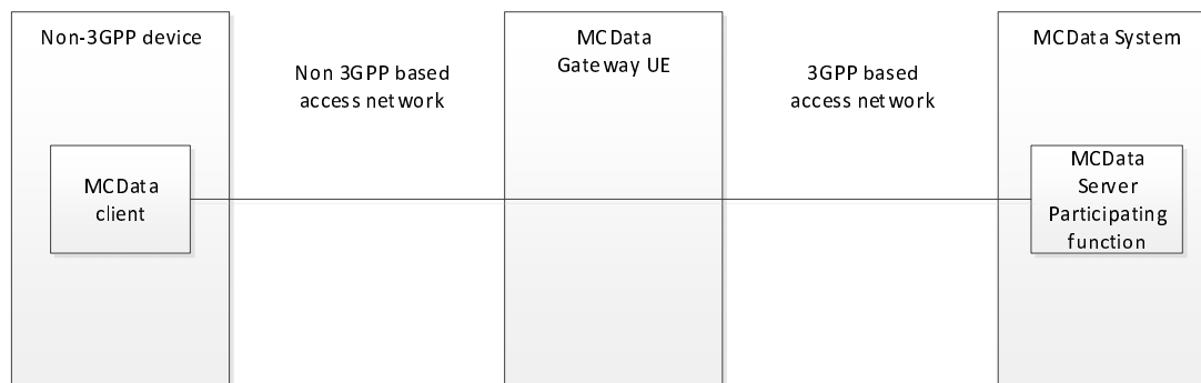
Figure 5.5.2-2: Relationship between non-3GPP device, MCDATA gateway UE and the MCDATA server with the MCDATA client located in the non-3GPP device
