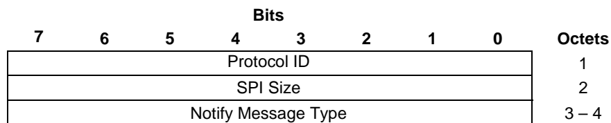
Figure 8.2.9.9-1: IKEV2_MULTIPLE_BEARER_PDN_CONNECTIVITY Notify Payload format
