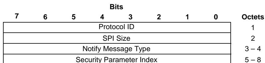
Figure 8.2.9.12-1: MODIFIED_BEARER Notify payload format
