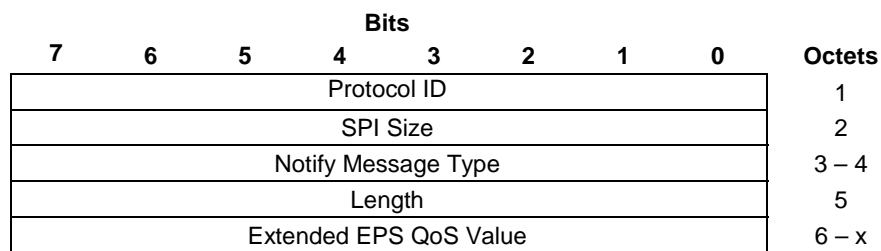
Figure 8.2.9.10A-1: EXTENDED_EPS_QOS Notify payload format
