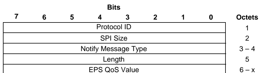
Figure 8.2.9.10-1: EPS_QOS Notify payload format
