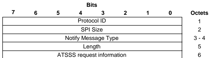
Figure 8.2.9.20-1: ATSSS_REQUEST Notify payload format
