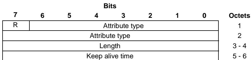
Figure F.3.3.1-1: FTT_KAT configuration attribute
