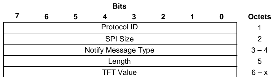
Figure 8.2.9.11-1: TFT Notify payload format
