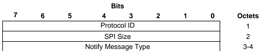
Figure 8.2.9.7-1: EMERGENCY_SUPPORT Notify Payload format
