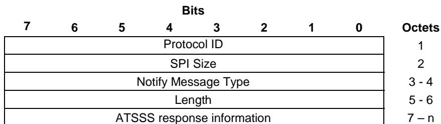
Figure 8.2.9.21-1: ATSSS_RESPONSE Notify payload format
