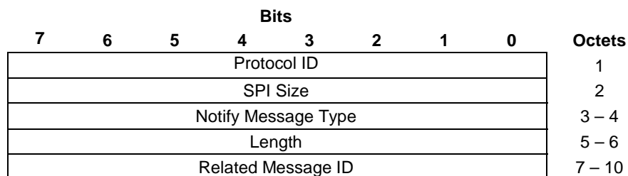
Figure 8.2.9.5-1: PTI Notify payload
