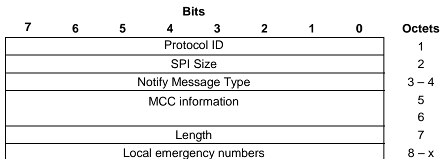
Figure 8.2.9.8-1: EMERGENCY_CALL_NUMBERS Notify payload
