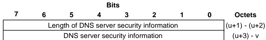
Figure 8.2.9.19-2: DNS server security parameter
