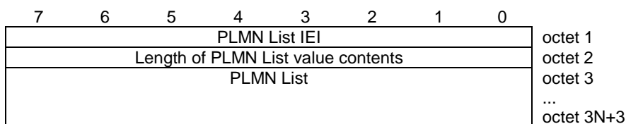
Figure H.2.4.2-1: PLMN List information element
