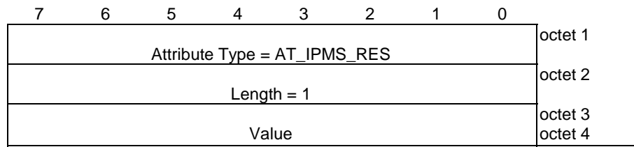
Figure 8.2.1.2: AT_IPMS_RES attribute.
