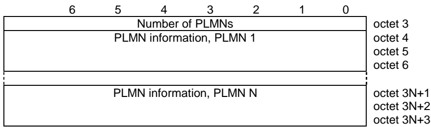
Figure H.2.4.2-1a: PLMN List
