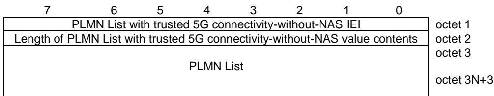
Figure H.2.4.5-1: PLMN List with trusted 5G connectivity-without-NAS information element
