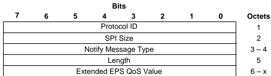
Figure 8.2.9.10A-1: EXTENDED_EPS_QOS Notify payload format
