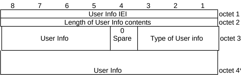
Figure 12.5.1.3.1: User Info information element
