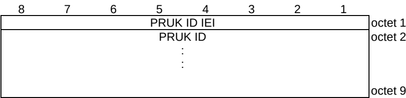
Figure 12.5.1.19.1: PRUK ID information element
