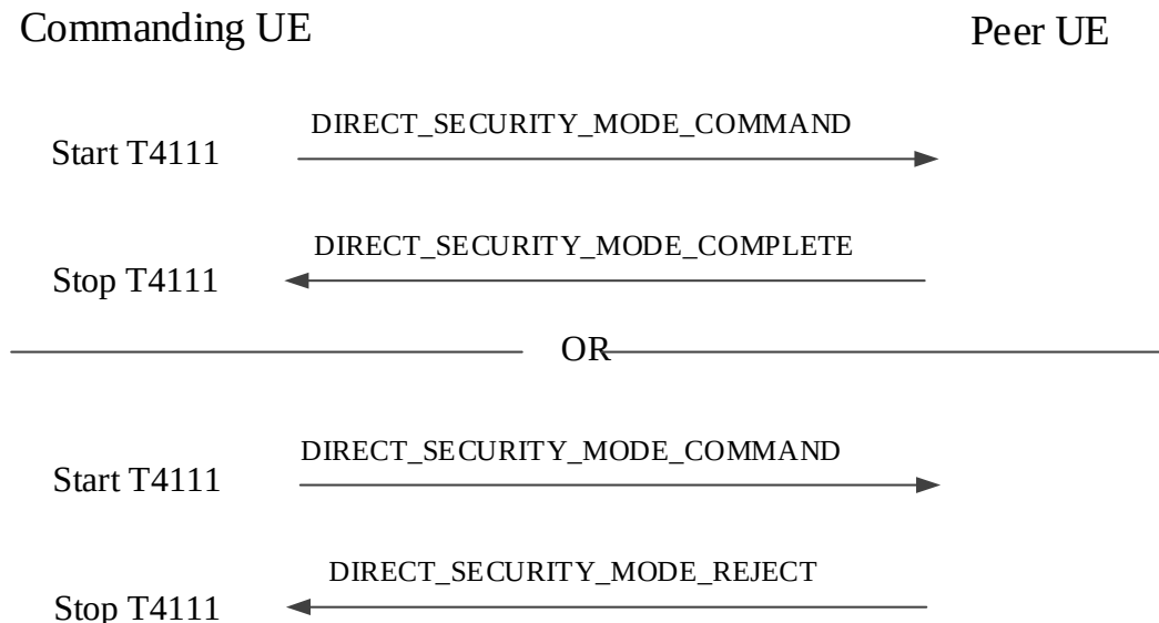
Figure 10.4.5.2.1: Direct Security mode control procedure
