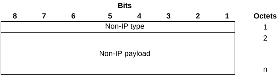
Figure 11.5.1: Non-IP data PDU format
