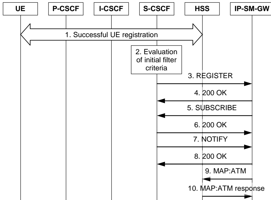
Figure B.3-1: IP-SM-GW registration signalling
