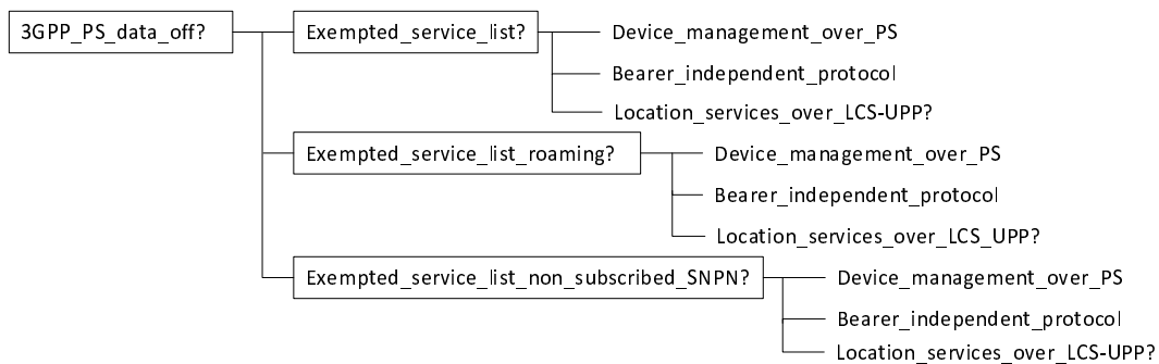
Figure 4-4: The NAS configuration Management Object (4 of 5)
