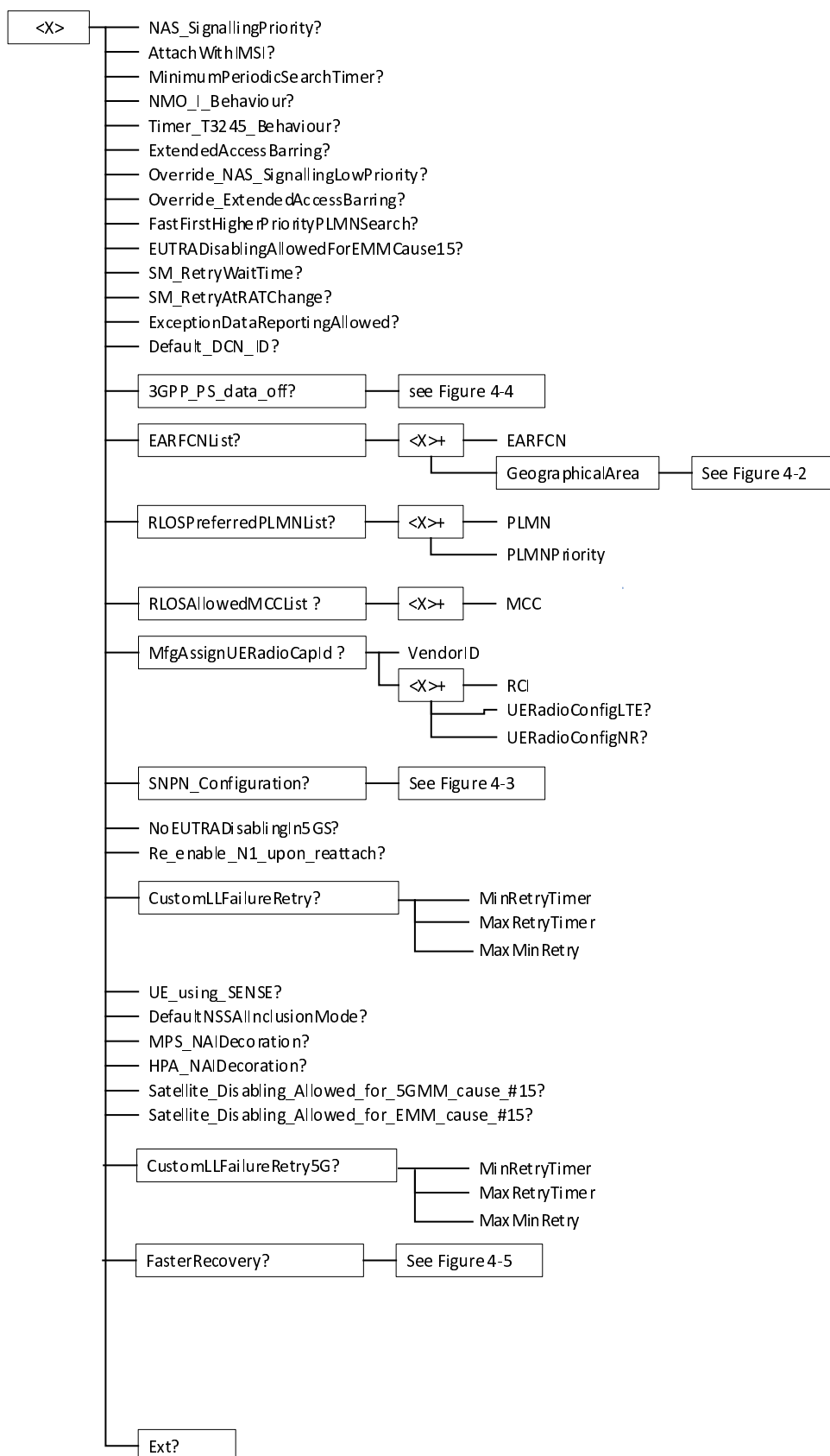
Figure 4-1: The NAS configuration Management Object (1 of 5)
