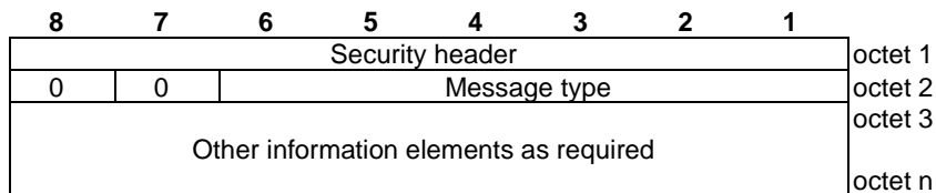
Figure 7.1.1-1: General message organization example for an unprotected AIoT NAS message
