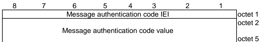
Figure 7.2.10-1: Message authentication code information element
