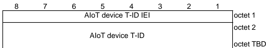
Figure 7.2.7-1: AIoT device T-ID information element
