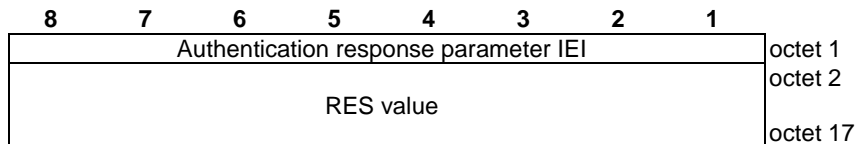
Figure 7.2.8-1 Authentication response parameter information element
