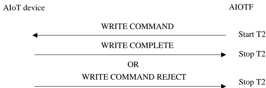
Figure 5.3.3.1.1: Write command procedure
