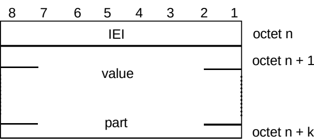
Figure I.2.2.4-6: Type 3 IE of format TV (k = 1, 2, ...)
