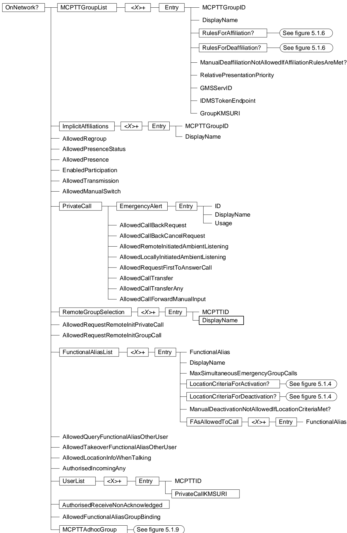
Figure 5.1.3: The MCPTT user profile MO (3 of 3)
