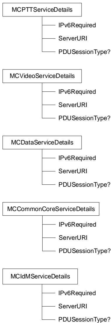
Figure 8.1.5: The MCS UE initial configuration MO (5 of 6)
