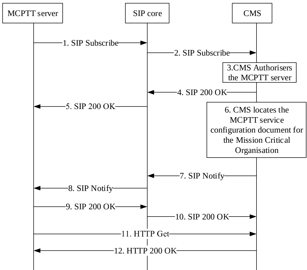
Figure A.2.3-1: MCPTT server subscribing to and obtaining the MCPTT service configuration document
