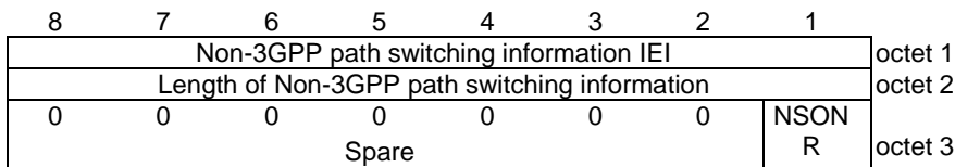
Figure 9.11.3.102.1: Non-3GPP path switching information information element
