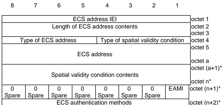
Figure 9.11.4.34.1: ECS address information element
