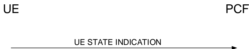
Figure D.2.2.2.1: UE-initiated UE state indication procedure
