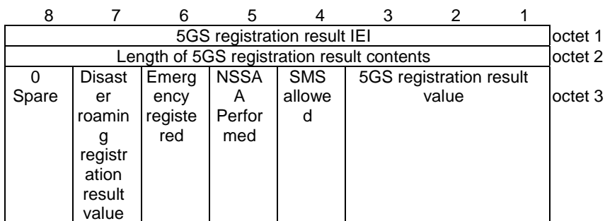
Figure 9.11.3.6.1: 5GS registration result information element
