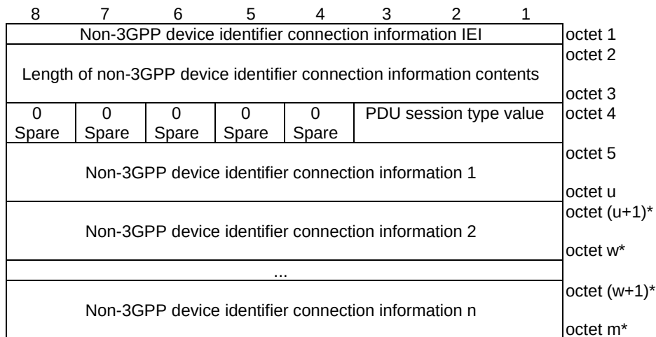
Figure 9.11.4.41.1: Non-3GPP device connection information information element
