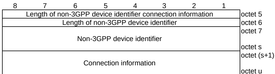
Figure 9.11.4.41.2: Non-3GPP device identifier connection information
