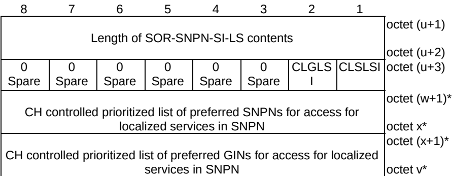
Figure 9.11.3.51.9A: SOR-SNPN-SI-LS Table 9.11.3.51.4A: SOR-SNPN-SI-LS
