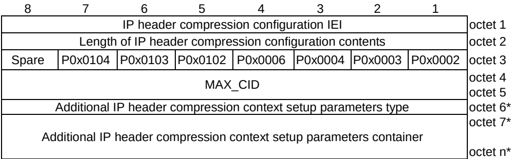
Figure 9.11.4.24.1: IP header compression configuration information element
