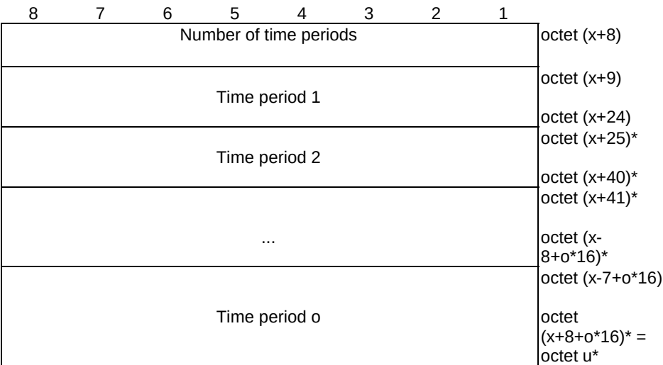
Figure 9.11.3.86.5: Time validity infomation
