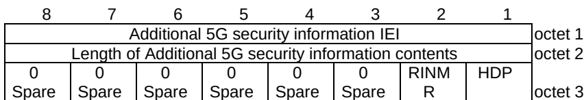
Figure 9.11.3.12.1: Additional 5G security information information element
