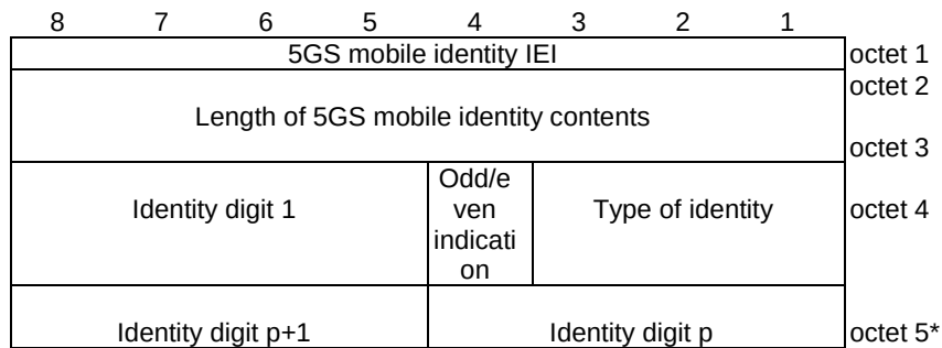
Figure 9.11.3.4.2: 5GS mobile identity information element for type of identity "IMEI" or "IMEISV"
