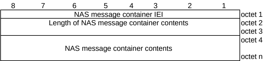
Figure 9.11.3.33.1: NAS message container information element
