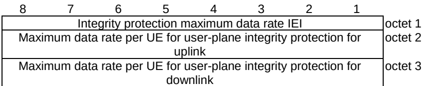
Figure 9.11.4.7.1: Integrity protection maximum data rate information element
