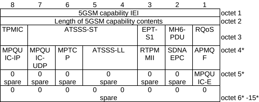
Figure 9.11.4.1.1: 5GSM capability information element
