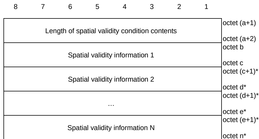
Figure 9.11.4.34.2: Spatial validity condition contents
