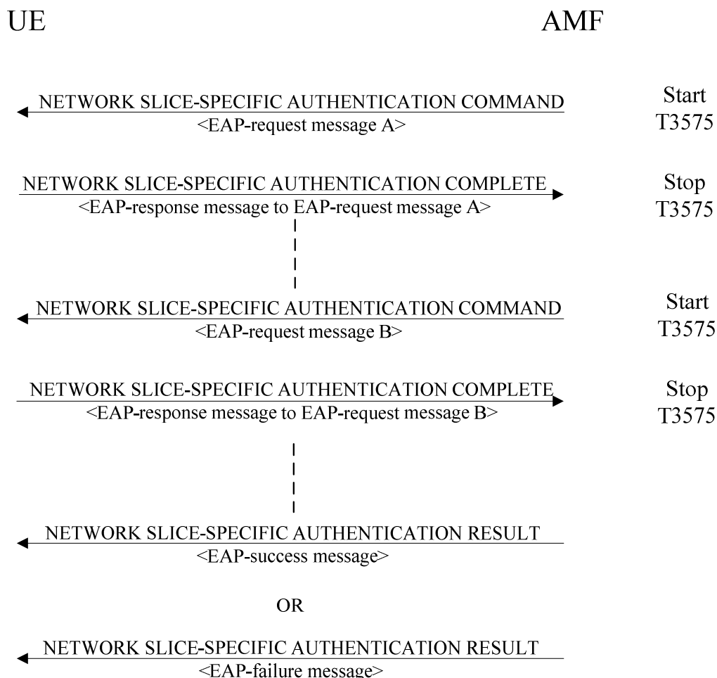
Figure 5.4.7.1.1: Network slice-specific authentication and authorization procedure
