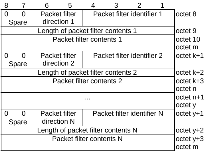
Figure 9.11.4.13.4: Packet filter list when the rule operation is "create new QoS rule", or "modify existing QoS rule and add packet filters" or "modify existing QoS rule and replace all packet filters"
