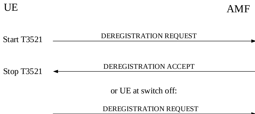
Figure 5.5.2.1.1: UE-initiated de-registration procedure
