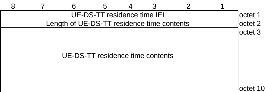
Figure 9.11.4.26.1: UE-DS-TT residence time information element
