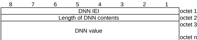
Figure 9.11.2.1B.1: DNN information element
