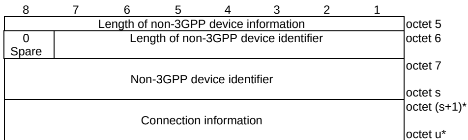
Figure 9.11.4.41.2: Non-3GPP device information
