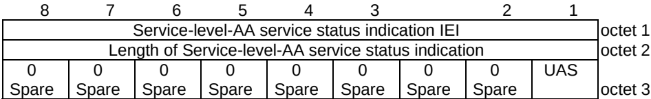
Figure 9.11.2.18.1: Service-level-AA-service-status indication information element
