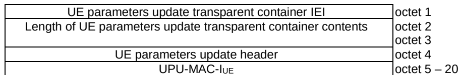
Figure 9.11.3.53A.5: UE parameters update transparent container information element for UE parameters update data type with value "1"
