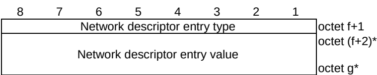
Figure D.6.8.4: Network descriptor entry
