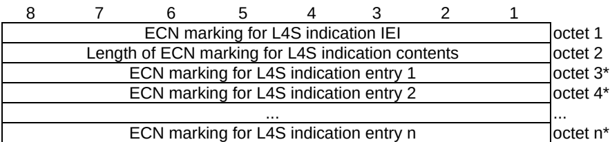
Figure 9.11.4.40.1: ECN marking for L4S indication information element
