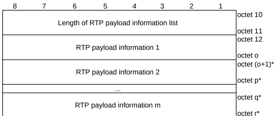
Figure 9.11.4.39.3: RTP payload information list
