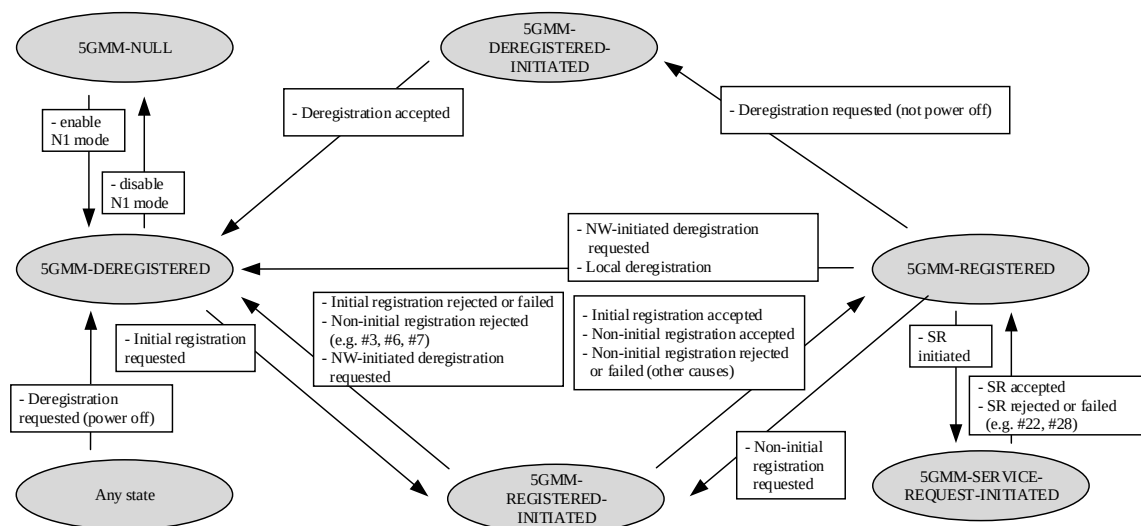
Figure 5.1.3.2.1.1.1: 5GMM main states in the UE
