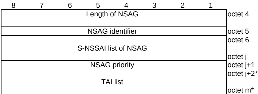
Figure 9.11.3.87.2: NSAG
