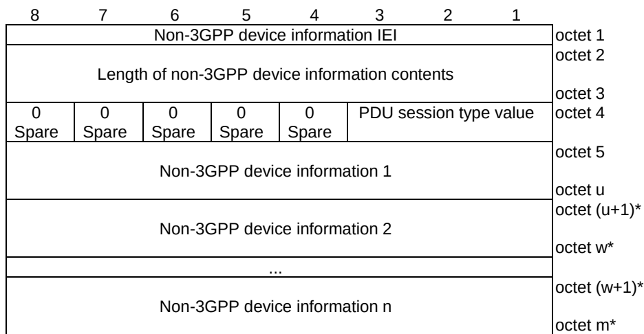
Figure 9.11.4.41.1: Non-3GPP device information information element
