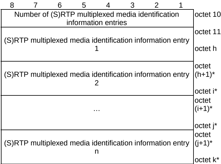
Figure 9.11.4.13.5: Value part of (S)RTP multiplexed media identification information component
