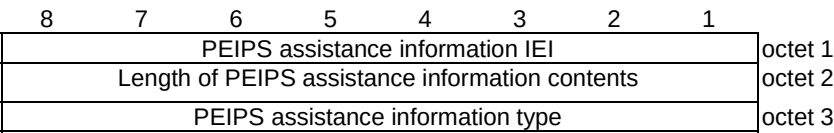
Figure 9.11.3.80.1: PEIPS assistance information information element
