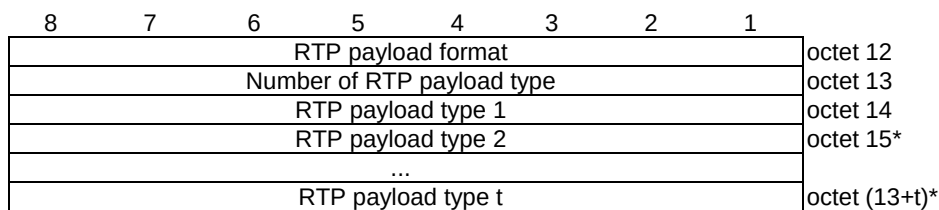
Figure 9.11.4.39.4: RTP payload information
