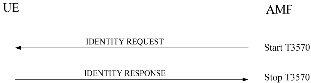
Figure 5.4.3.2.1: Identification procedure
