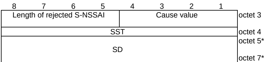
Figure 9.11.3.46.2: Rejected S-NSSAI
