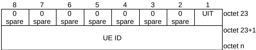
Figure 9.11.3.89.2: UE identity
