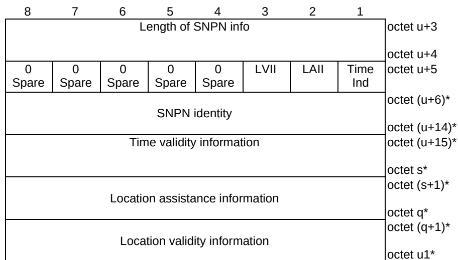
Figure 9.11.3.51.10B: SNPN info
