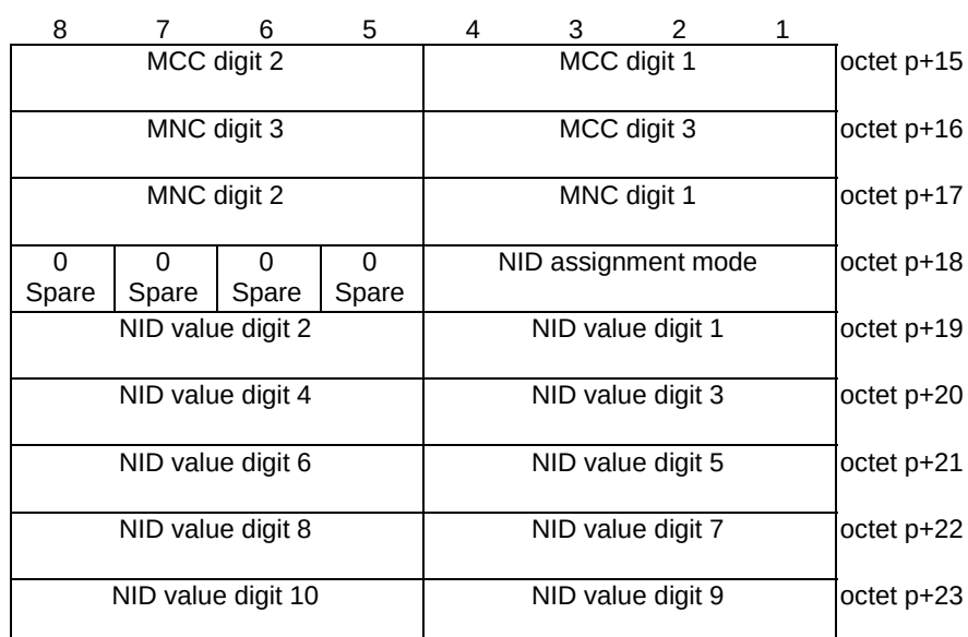
Figure 9.11.3.51.11: SNPN identity
