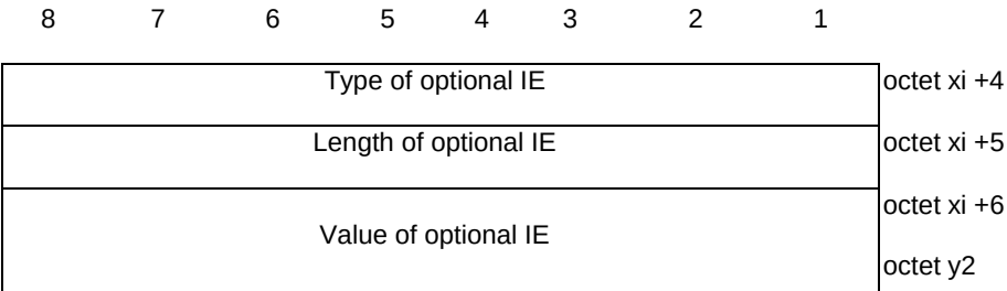
Figure 9.11.3.39.4: Optional IE
