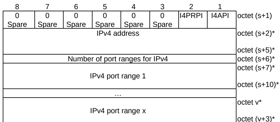
Figure 9.11.4.41.3: Connection information when PDU session type value = "IPv4"
