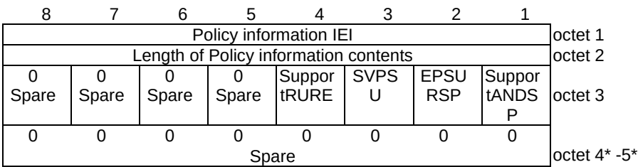
Figure D.6.5.1: UE policy classmark information element
