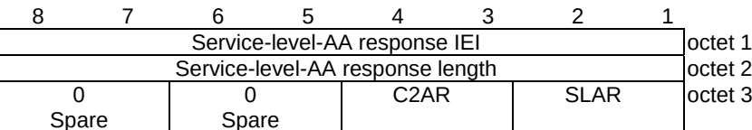
Figure 9.11.2.14.1: Service-level-AA response information element
