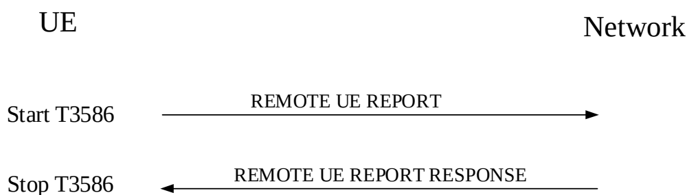
Figure 6.6.2.2.1: Remote UE report procedure
