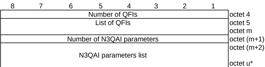
Figure 9.11.4.36.2: N3QAI
