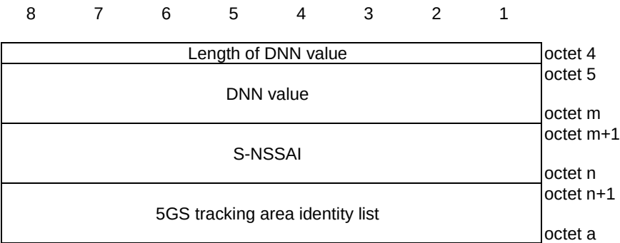
Figure 9.11.3.96.2: LADN
