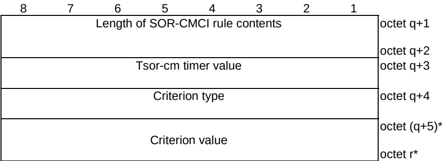
Figure 9.11.3.51.8: SOR-CMCI rule
