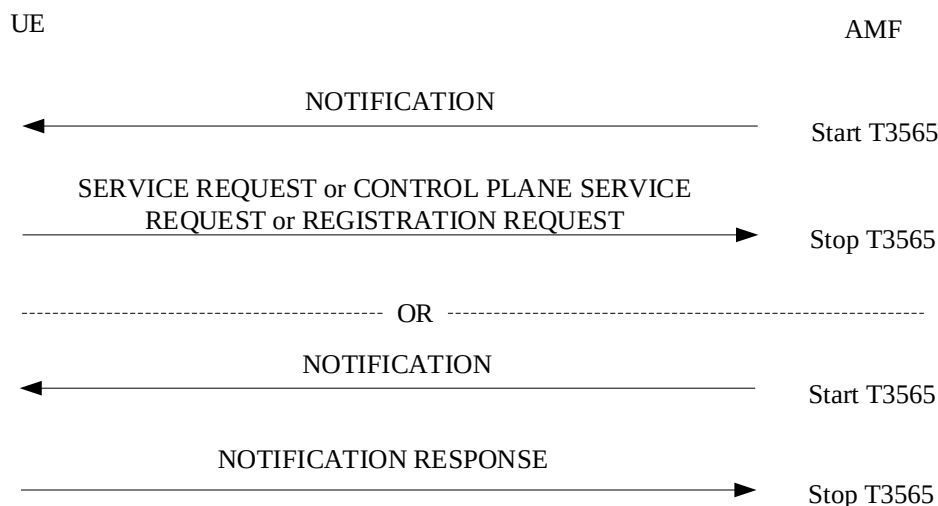
Figure 5.6.3.2.1: Notification procedure
