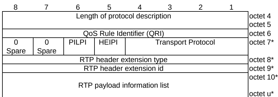
Figure 9.11.4.39.2: Protocol description
