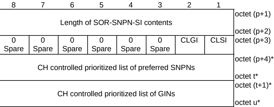
Figure 9.11.3.51.9: SOR-SNPNI-SI
