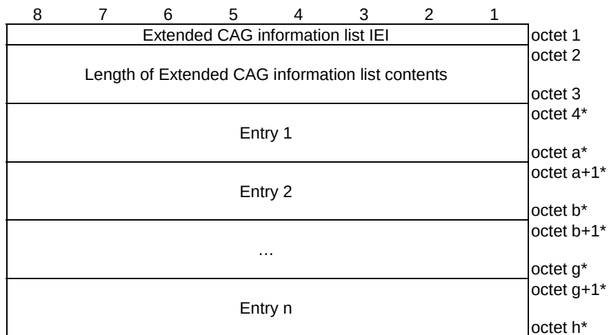
Figure 9.11.3.86.1: Extended CAG information list information element
