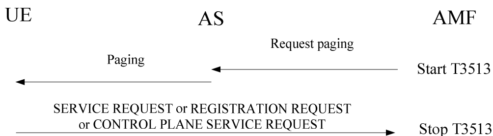
Figure 5.6.2.2.1.1: Paging procedure
