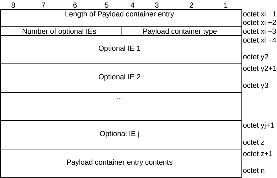
Figure 9.11.3.39.3: Payload container entry
