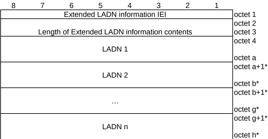
Figure 9.11.3.96.1: Extended LADN information information element
