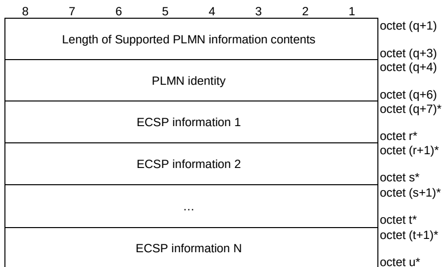
Figure 9.11.4.34.5: Supported PLMN information contents
