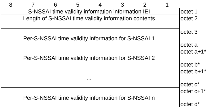
Figure 9.11.3.101.1: S-NSSAI time validity information information element
