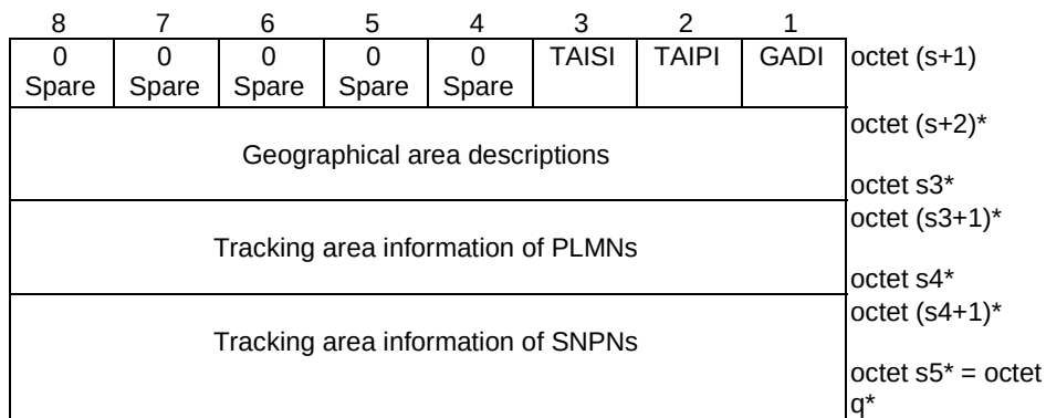
Figure 9.11.3.51.11B: Location assistance information
