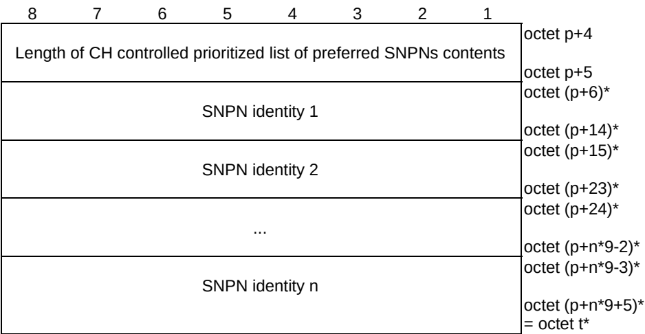
Figure 9.11.3.51.10: CH controlled prioritized list of preferred SNPNs
