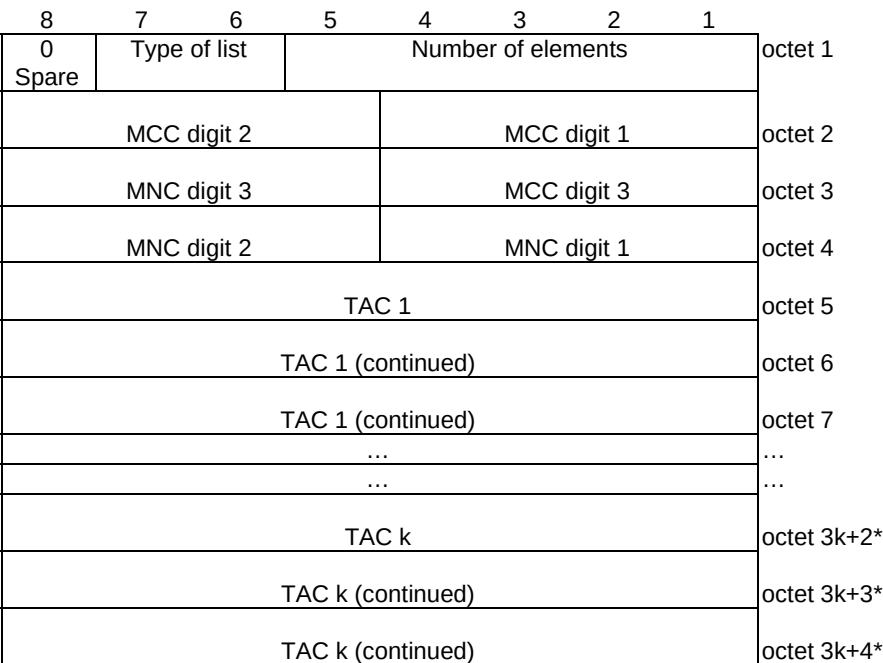
Figure 9.11.3.9.2: Partial tracking area identity list – type of list = "00"
