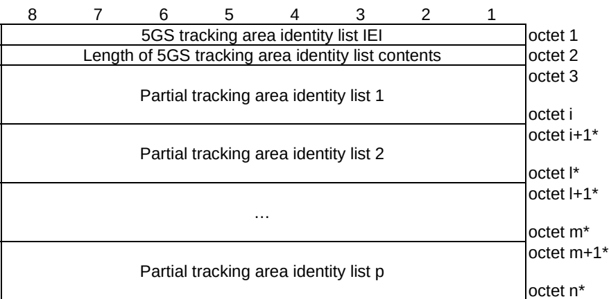
Figure 9.11.3.9.1: 5GS tracking area identity list information element
