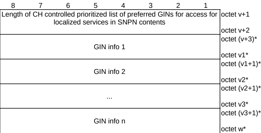
Figure 9.11.3.51.12A: CH controlled prioritized list of preferred GINs for access for localized services in SNPN
