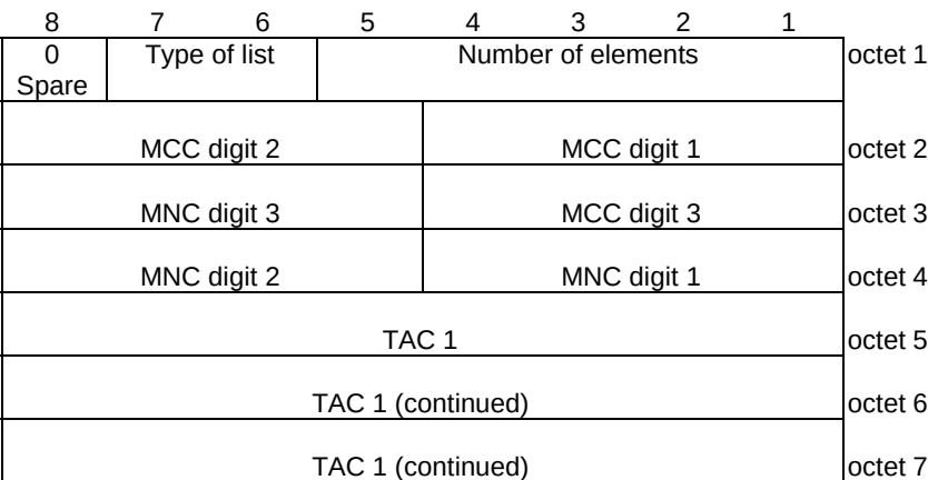
Figure 9.11.3.9.3: Partial tracking area identity list – type of list = "01"
