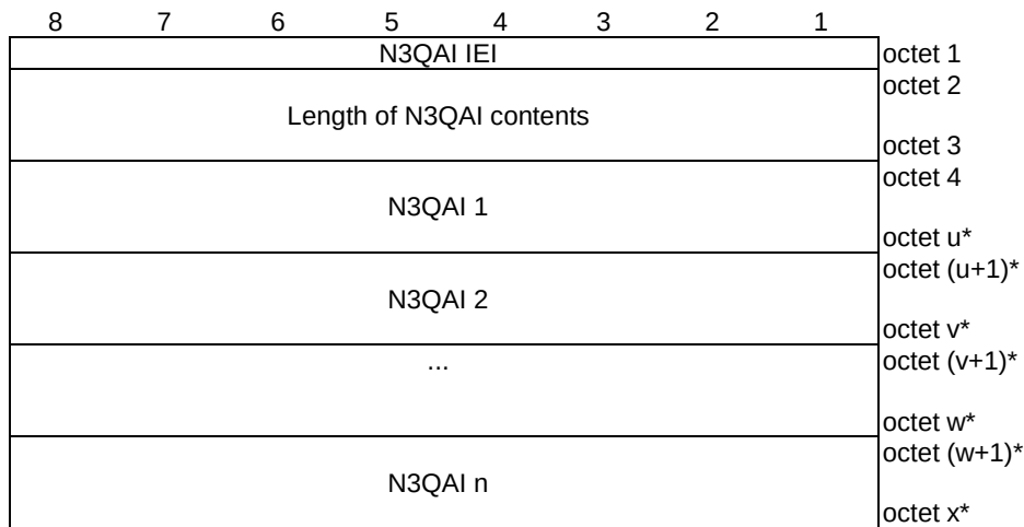
Figure 9.11.4.36.1: N3QAI information element
