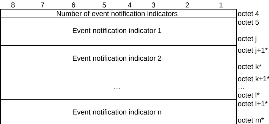
Figure 9.11.3.39.1A: Payload container contents with Payload container type "Event notification"
