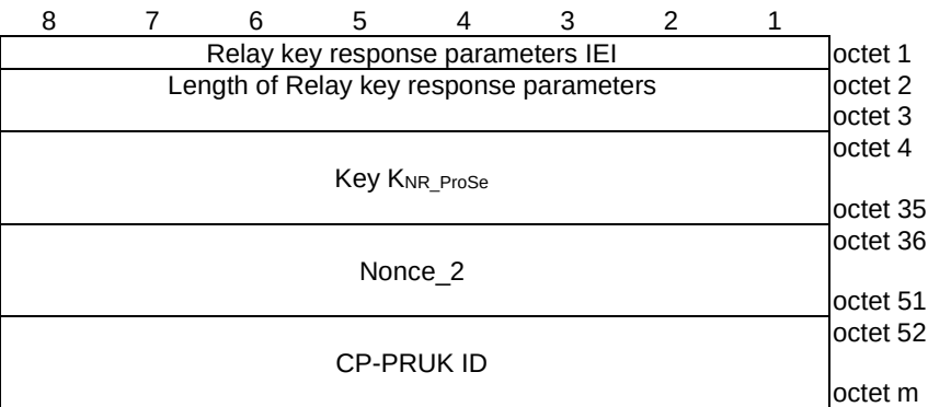
Figure 9.11.3.90.1: Relay key response parameters information element
