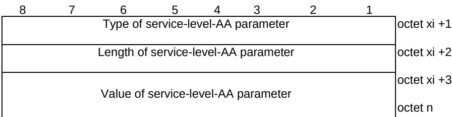
Figure 9.11.2.10.3: Service-level-AA parameter (when the type of service-level-AA parameter field contains an IEI of a type 4 information element as specified in 3GPP TS 24.007 [11])
