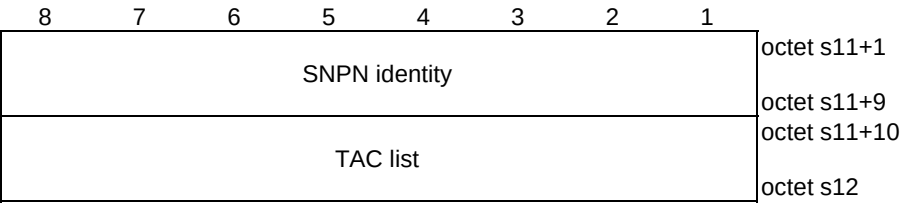
Figure 9.11.3.51.11H: Tracking area information of SNPN
