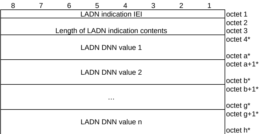
Figure 9.11.3.29.1: LADN indication information element
