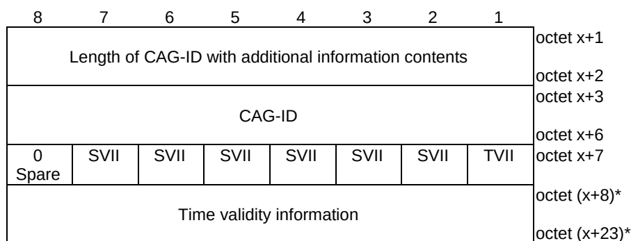
Figure 9.11.3.86.4: CAG-ID with additional information
