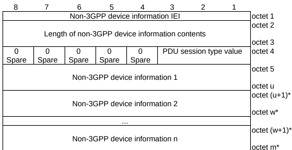
Figure 9.11.4.41.1: Non-3GPP device information information element
