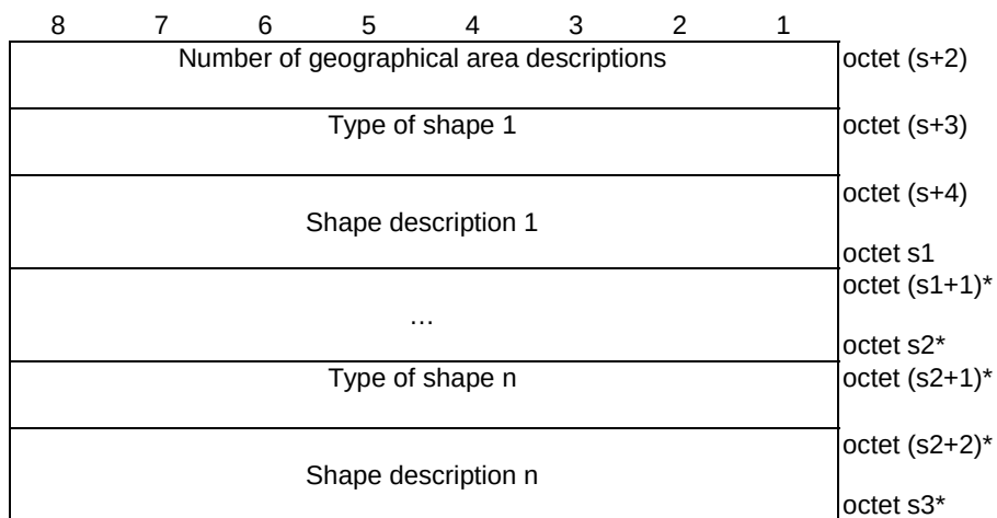
Figure 9.11.3.51.11C: Geographical area descriptions
