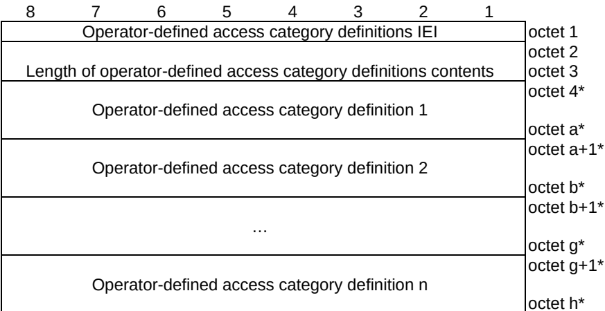
Figure 9.11.3.38.1: Operator-defined access category definitions information element
