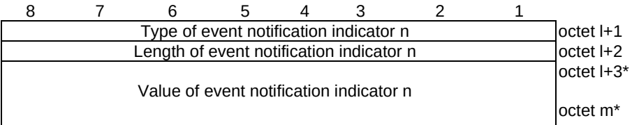
Figure 9.11.3.39.1B: Even notification indicator n
