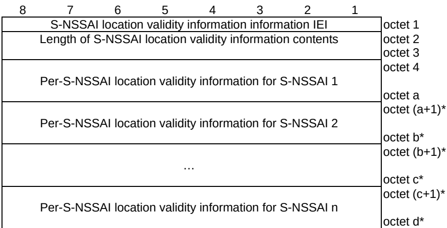
Figure 9.11.3.100.1: S-NSSAI location validity information information element
