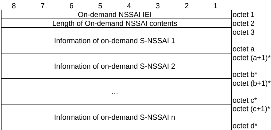
Figure 9.11.3.108.1: On-demand NSSAI information element
