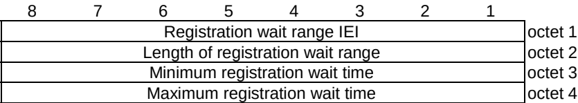
Figure 9.11.3.84.1: Registration wait range information element
