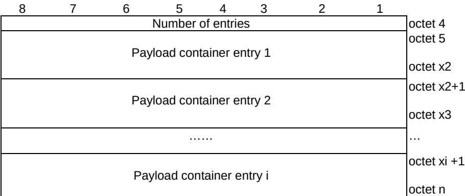
Figure 9.11.3.39.2: Payload container contents with Payload container type "Multiple payloads"
