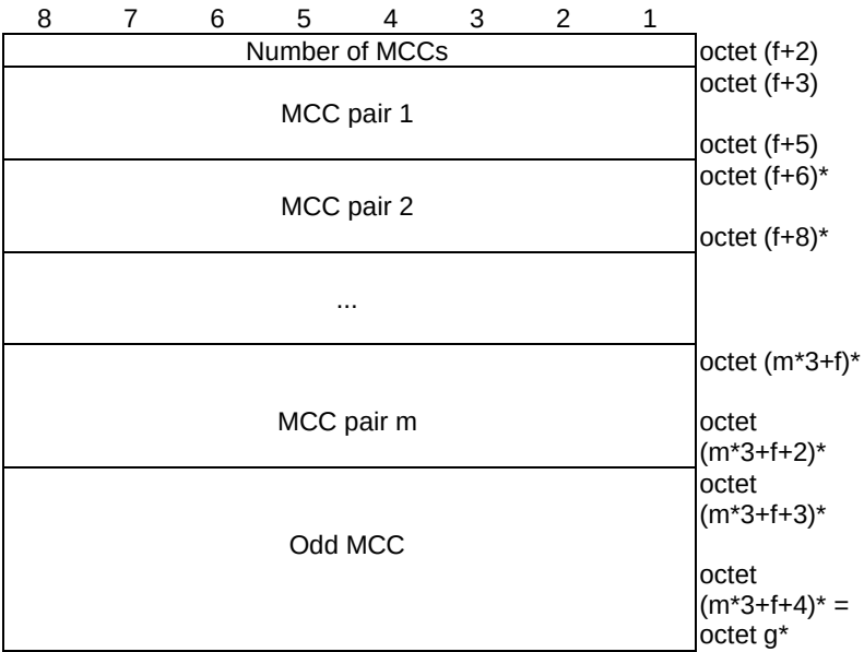
Figure D.6.8.7: Network descriptor entry value for network descriptor entry type set to "one or more MCCs"
