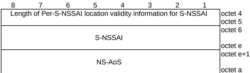
Figure 9.11.3.100.2: Per-S-NSSAI location validity information for S-NSSAI
