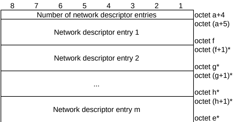
Figure D.6.8.3: Network descriptor
