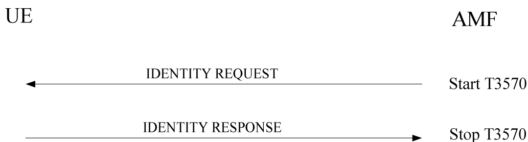
Figure 5.4.3.2.1: Identification procedure
