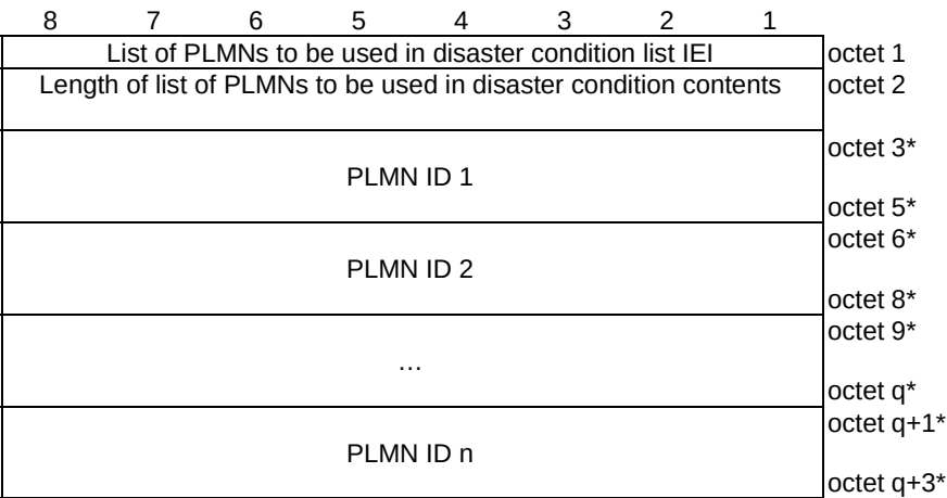
Figure 9.11.3.83.1: List of PLMNs to be used in disaster condition information element
