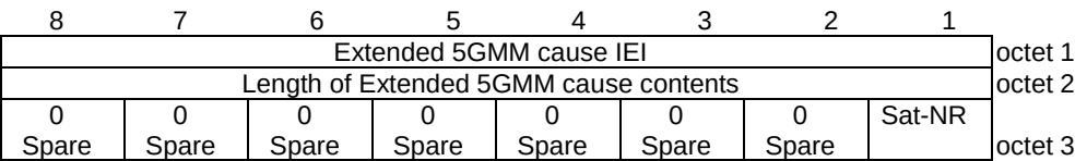
Figure 9.11.3.109.1: Extended 5GMM cause information element
