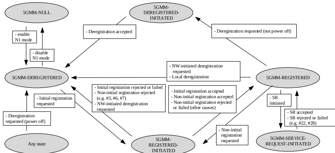
Figure 5.1.3.2.1.1.1: 5GMM main states in the UE
