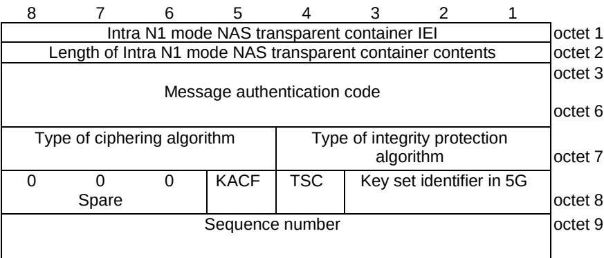
Figure 9.11.2.6.1: Intra N1 mode NAS transparent container information element
