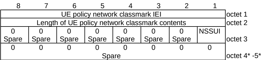
Figure D.6.7.1: UE policy network classmark information element
