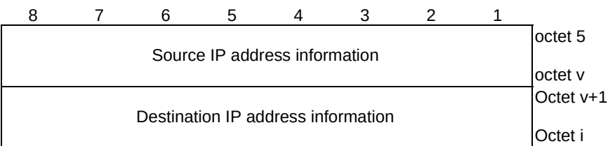
Figure 9.11.4.30.4: multicast MBS session ID for Type of multicast MBS session ID = "Source specific IP multicast address for IPv4" or "Source specific IP multicast address for IPv6"
