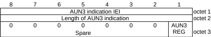
Figure 9.11.3.104.1: AUN3 indication information element
