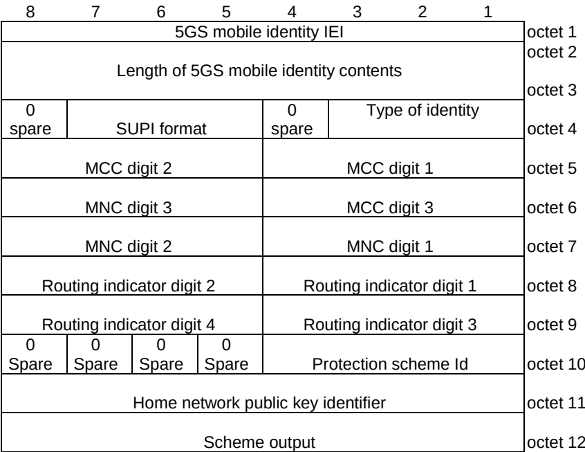
Figure 9.11.3.4.3: 5GS mobile identity information element for type of identity "SUCI" and SUPI format "IMSI"
