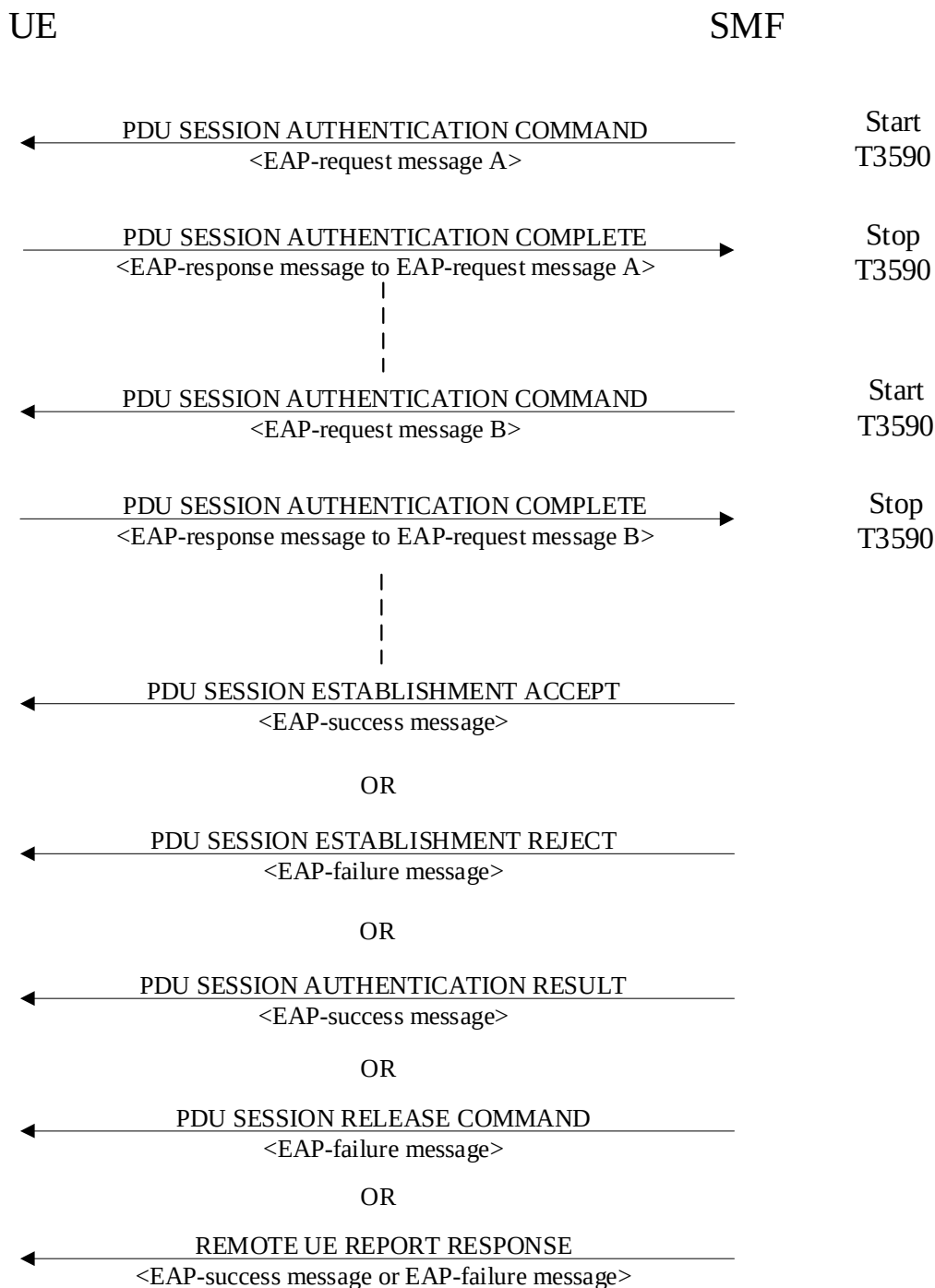
Figure 6.3.1.1: PDU session authentication and authorization procedure
