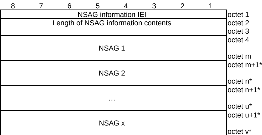
Figure 9.11.3.87.1: NSAG information information element
