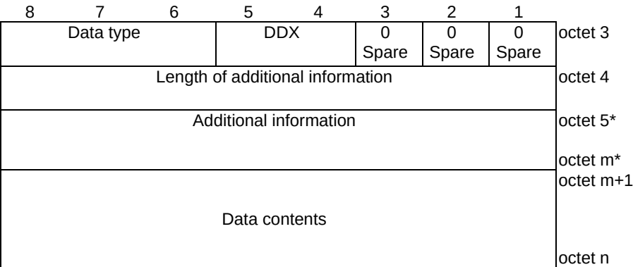
Figure 9.11.3.18B.3: Clot small data container contents for Data type "Location services message container"
