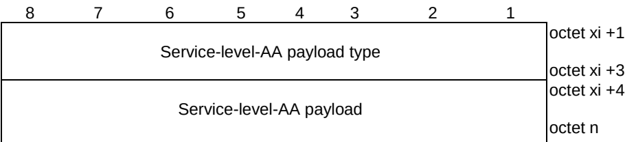
Figure 9.11.2.10.5: Service-level-AA parameter (when Service-level-AA payload type and its associated Service-level-AA payload are included in the Service-level-AA container contents)
