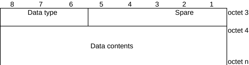
Figure 9.11.3.18B.4: Clot small data container contents for Data type "SMS"
