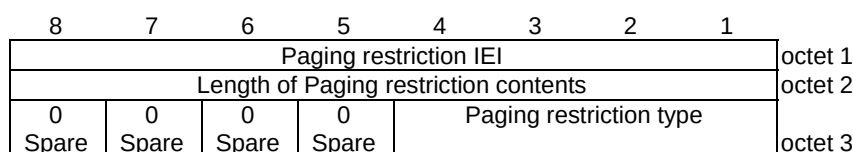
Figure 9.11.3.77.1: Paging restriction information element for Paging restriction type = "All paging is restricted" and for Paging restriction type = "All paging is restricted except voice"
