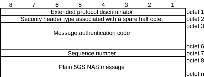
Figure 9.1.1.2: General message organization example for a security protected 5GS NAS message
