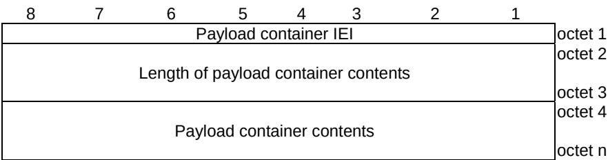
Figure 9.11.3.39.1: Payload container information element
