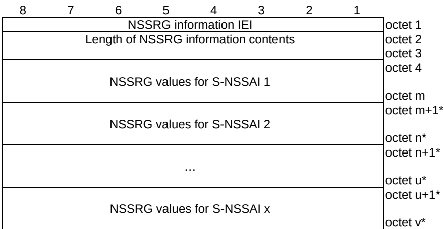
Figure 9.11.3.82.1: NSSRG information information element
