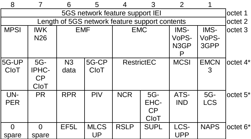
Figure 9.11.3.5.1: 5GS network feature support information element
