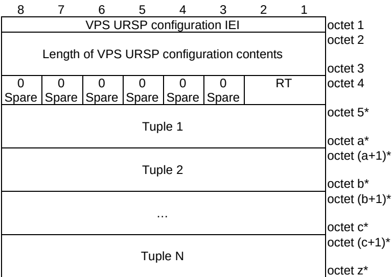
Figure D.6.8.1: VPS URSP configuration information element
