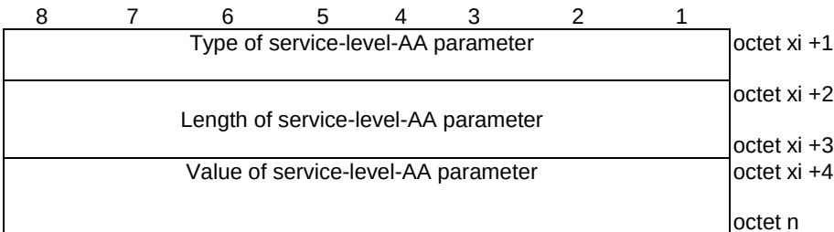
Figure 9.11.2.10.4: Service-level-AA parameter (when the type of service-level-AA parameter field contains an IEI of a type 6 information element as specified in 3GPP TS 24.007 [11])
