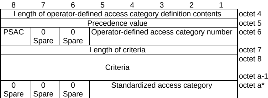
Figure 9.11.3.38.2: Operator-defined access category definition
