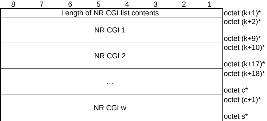
Figure 9.11.4.31.6: NR CGI list
