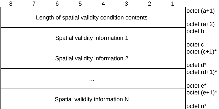
Figure 9.11.4.34.2: Spatial validity condition contents
