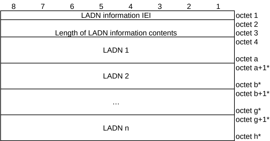
Figure 9.11.3.30.1: LADN information information element
