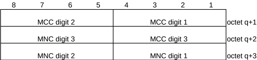
Figure 9.11.3.83.2: PLMN ID n
