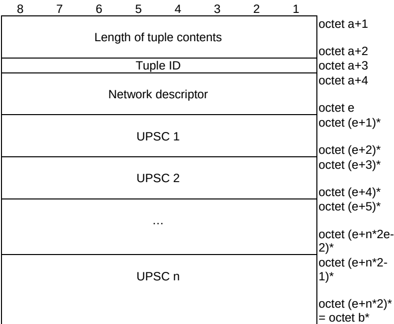
Figure D.6.8.2: Tuple
