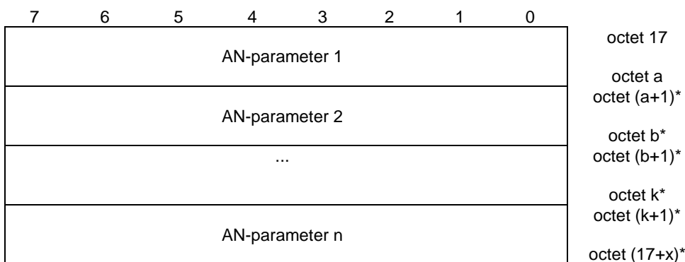
Figure 9.3.2.2.2.2: AN-parameters field
