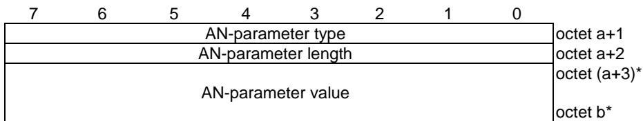
Figure 9.3.2.2.3: AN-parameter field
