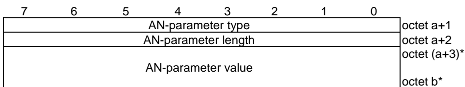
Figure 9.3.2.2.2-3: AN-parameter field
