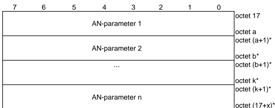
Figure 9.3.2.2.2-2: AN-parameters field
