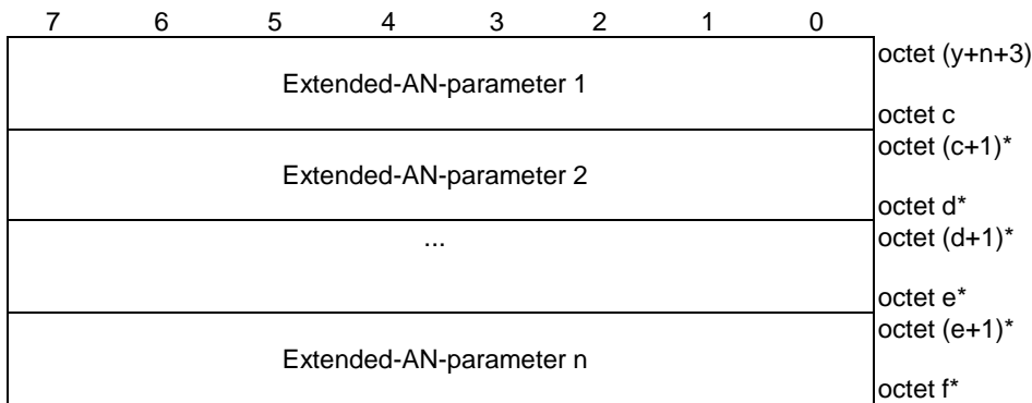
Figure 9.3.2.2.2-4: Extended-AN-parameters field
