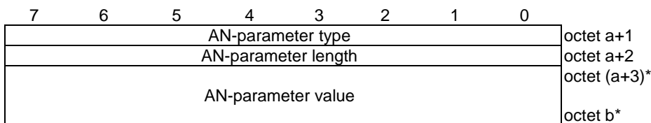
Figure 9.3.2.2.2-3: AN-parameter field
