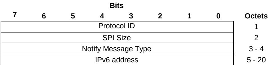
Figure 9.3.1.5-1: UP_IP6_ADDRESS Notify payload format
