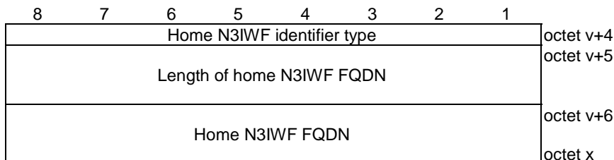
Figure 5.3.3.3.3: Home N3IWF identifier entry (Home N3IWF identifier type = "FQDN")
