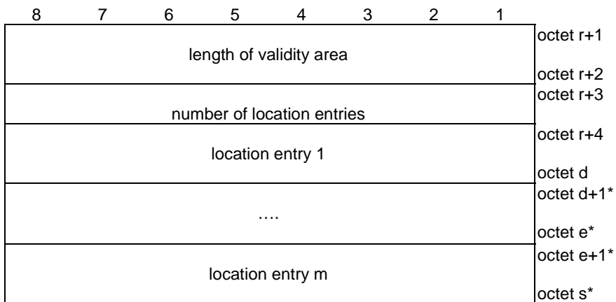
Figure 5.3.2.5: Validity area
