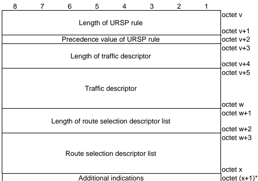
Figure 5.2.2: URSP rule
