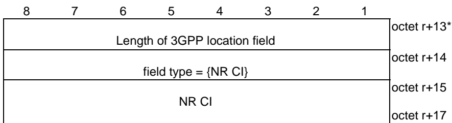
Figure 5.3.2.14: 3GPP location field {field type = NR CI}
