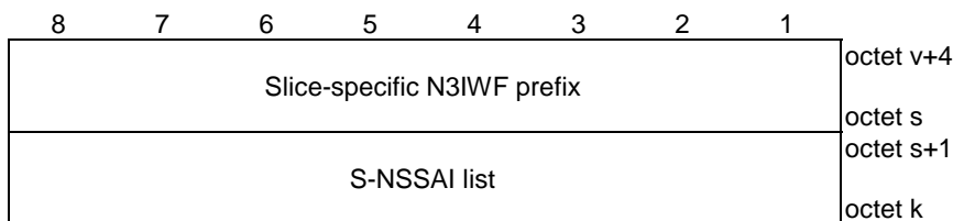
Figure 5.3.3.6.2: slice-specific N3IWF prefix entry
