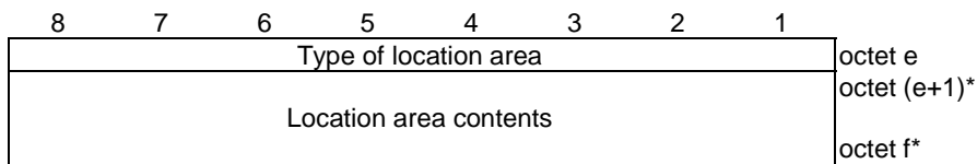
Figure 5.2.6: Location area
