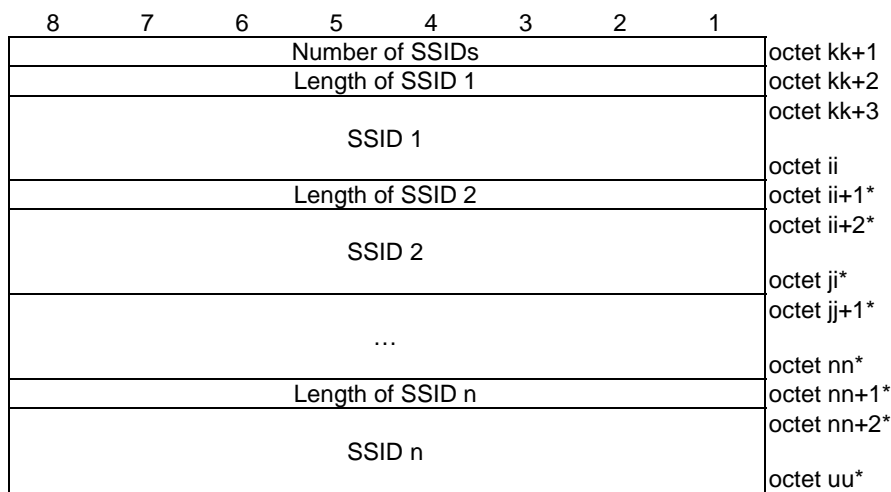
Figure 5.3.2.21: SSID list
