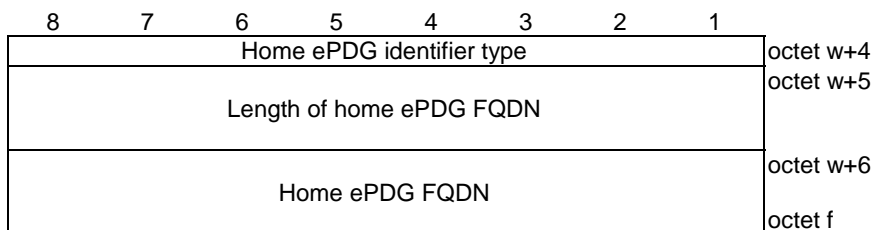
Figure 5.3.3.4.3: Home ePDG identifier entry (Home ePDG identifier type = "FQDN")
