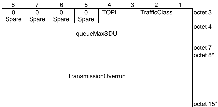
Figure 9.22.2: queueMaxSDUEntry
