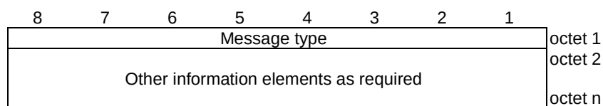
Figure 8.2.1-2: General message organization example
