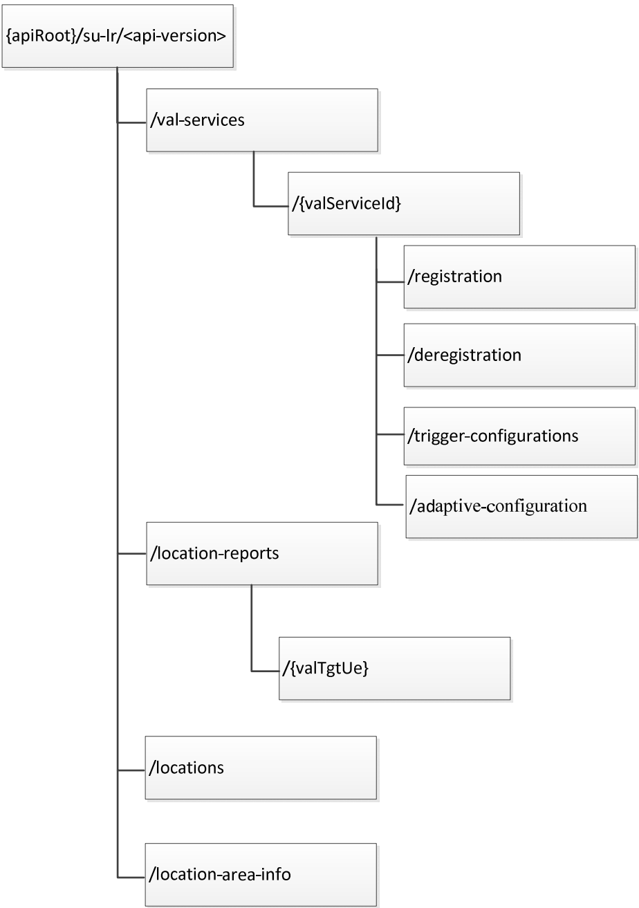
Figure B.3.1.2.1-1: Resource URI structure of the SU_LocationReporting API provided by SLM-S
