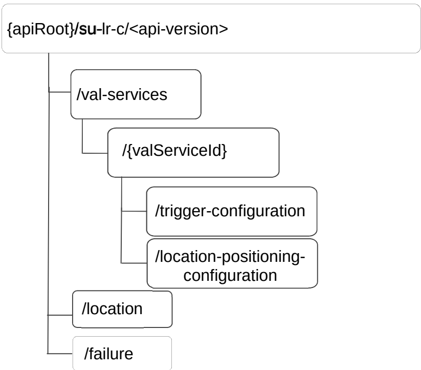
Figure B.4.1.2.1-1: Resource URI structure of the SU_LocationReporting API provided by SLM-C
