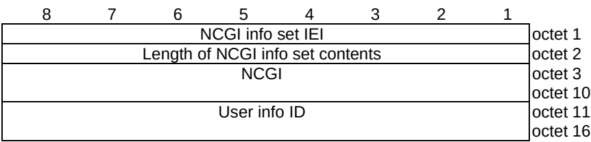
Figure 11.2.25.1: NCGI info set information element
