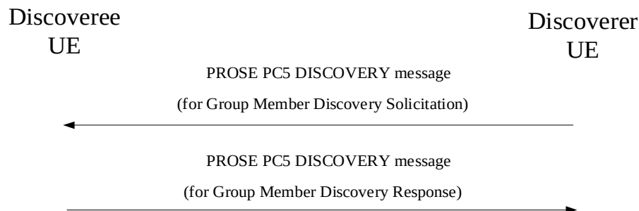
Figure 6.2.15.2.2.4.1: Discoveree UE procedure for group member discovery
