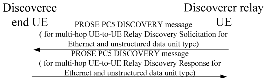
Figure 8a.2.1.3.3.4.2.1: Discoveree end UE procedure for multi-hop layer-3 UE-to-UE relay discovery
