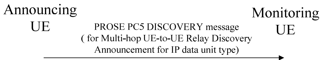
Figure 8c.2.1.2.2.2.2.1: Announcing UE procedure for multi-hop layer-3 UE-to-UE relay discovery for IP data unit type
