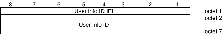
Figure 11.2.7.1: User info ID information element
