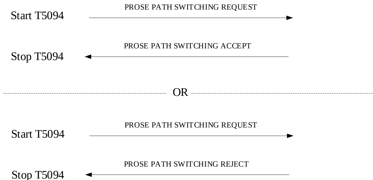
Figure 7.7.3.2.1: Path switching procedure from the direct communication path over PC5 to the direct communication path over Uu
