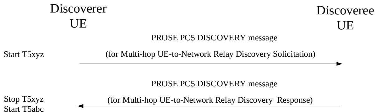
Figure 8b.2.1.3.2.3.1: Discoverer intermediate UE procedure for multi-hop UE-to-network Relay discovery
