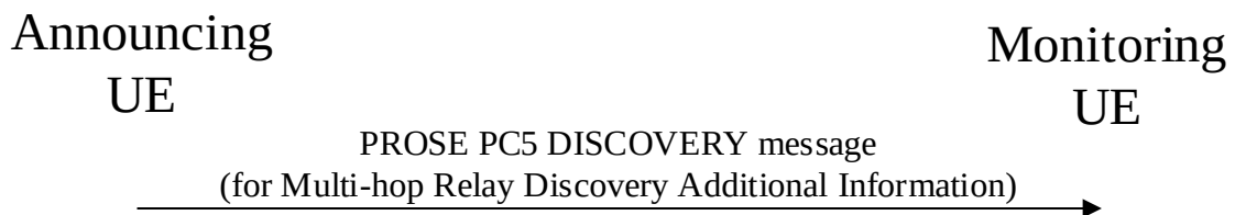
Figure 8b.2.1.2.4.3-1: ProSe intermediate UE-to-network relay UE procedure for announcing multi-hop UE-to-network relay discovery additional information
