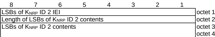
Figure 11.3.53.1: LSBs of K_{\text{NRP}} ID 2 information element
