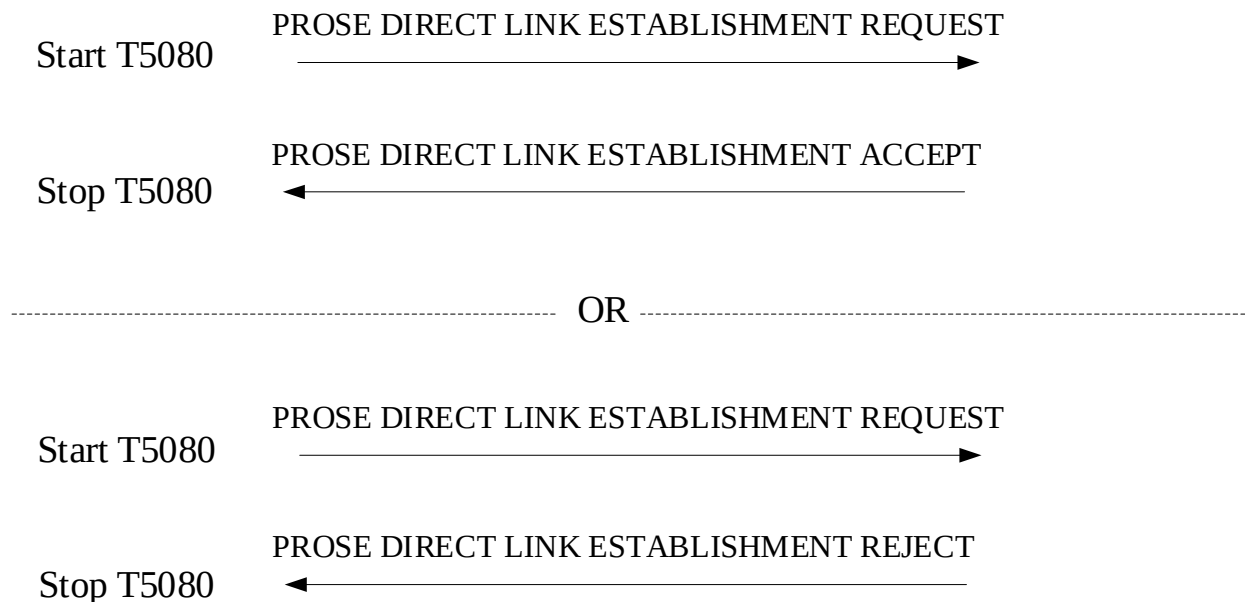
Figure 7.2.2.2.1: UE oriented 5G ProSe direct link establishment procedure
