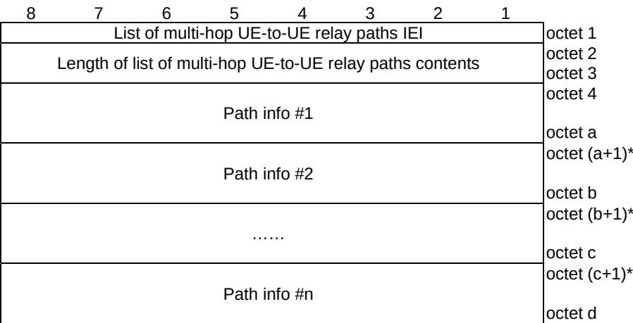
Figure 11.2.24.1: List of multi-hop UE-to-UE relay paths information element
