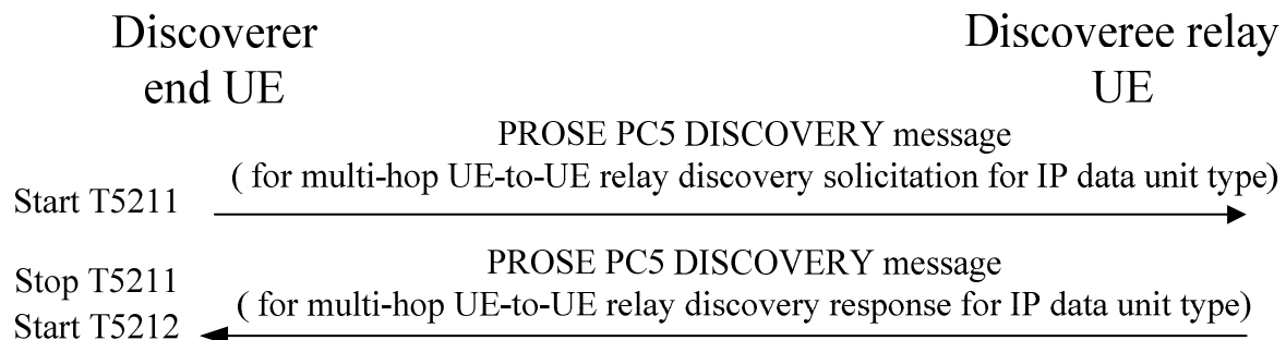
Figure 8c.2.1.2.3.2.2.1: Discoverer end UE procedure for multi-hop layer-3 UE-to-UE Relay discovery
