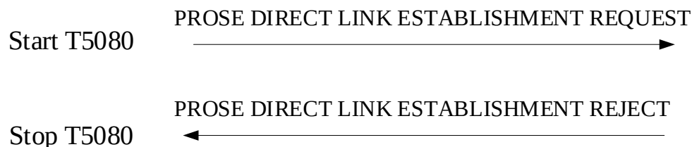
Figure 7.2.2.2.1: UE oriented 5G ProSe direct link establishment procedure
