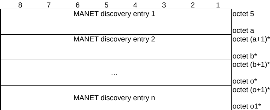
Figure 11.8.1.2: List of multi-hop UE-to-UE discovery info
