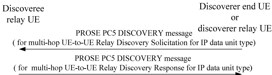
Figure 8c.2.1.3.4.2.1: Discoverer relay UE procedure for multi-hop layer-3 UE-to-UE relay discovery
