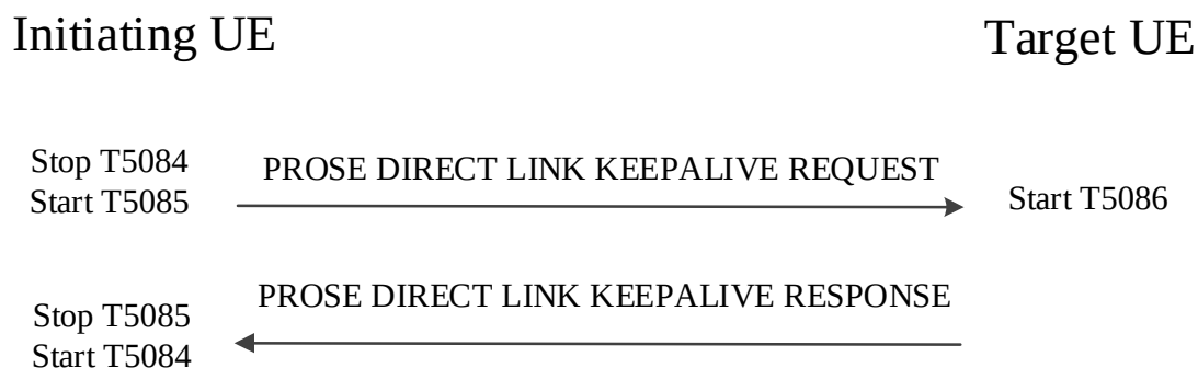
Figure 7.2.5.2.1: 5G ProSe direct link keep-alive procedure
