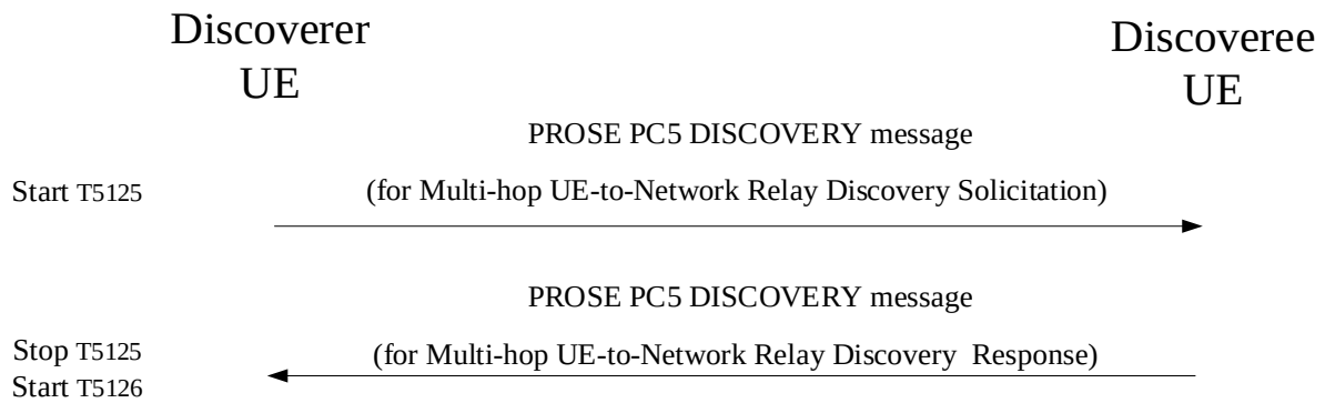
Figure 8b.2.1.3.2.2.1: Discoverer remote UE procedure for multi-hop UE-to-network Relay discovery
