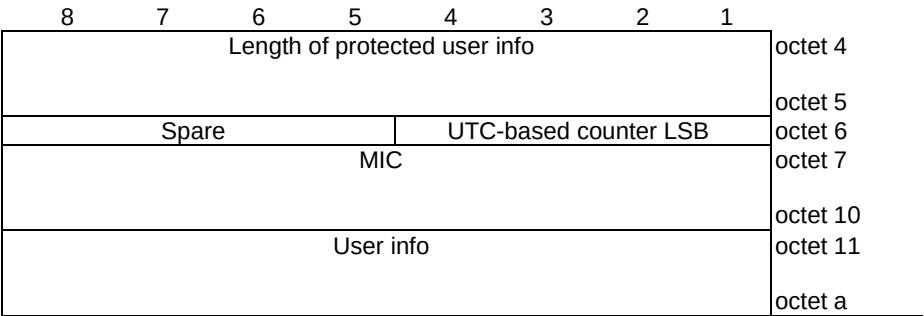
Figure 11.2.17.3: Protected user info
