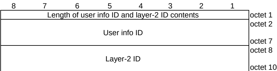
Figure 11.3.48.2: User info ID and layer-2 ID
