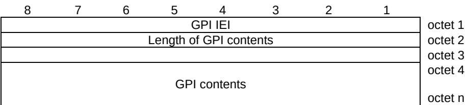
Figure 11.3.35.1: GPI information element
