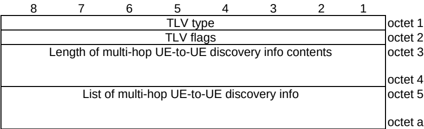
Figure 11.8.1.1: Multi-hop UE-to-UE discovery info parameter
