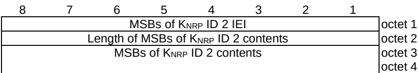
Figure 11.3.52.1: MSBs of K NRP ID 2 information element
