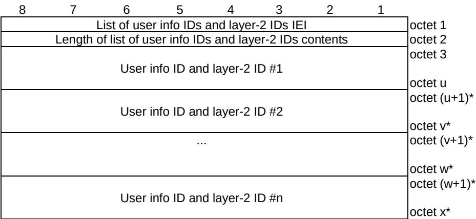
Figure 11.3.48.1: List of user info IDs and layer-2 IDs information element
