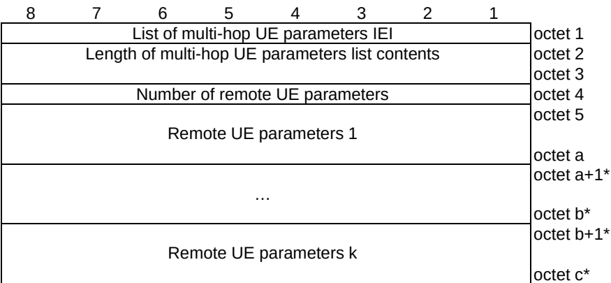
Figure 11.3.58.1: List of multi-hop remote UE parameters information element
