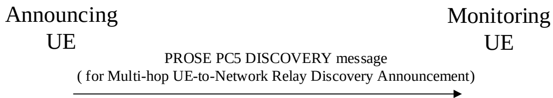
Figure 8b.2.1.2.3.3-1: ProSe multi-hop remote UE procedure for multi-hop UE-to-network relay discovery monitoring
