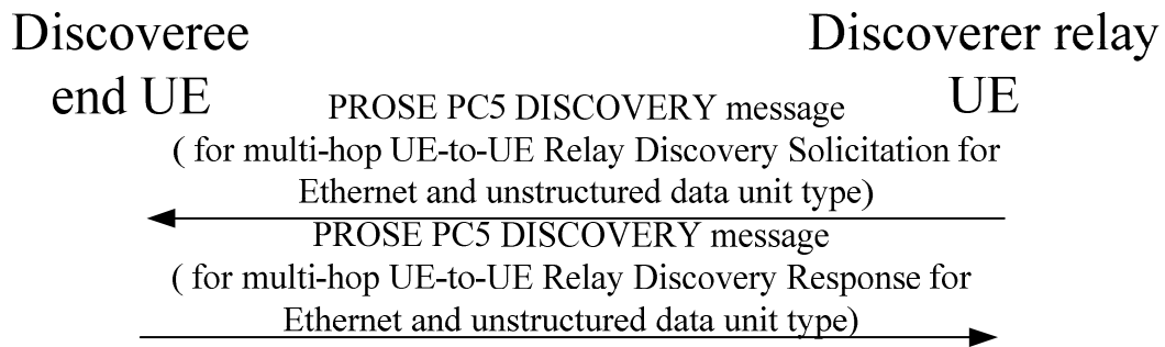
Figure 8c.2.1.3.3.4.2.1: Discoveree end UE procedure for multi-hop layer-3 UE-to-UE relay discovery
