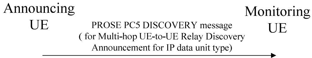
Figure 8c.2.1.2.2.2.1: Announcing UE procedure for multi-hop layer-3 UE-to-UE relay discovery for IP data unit type
