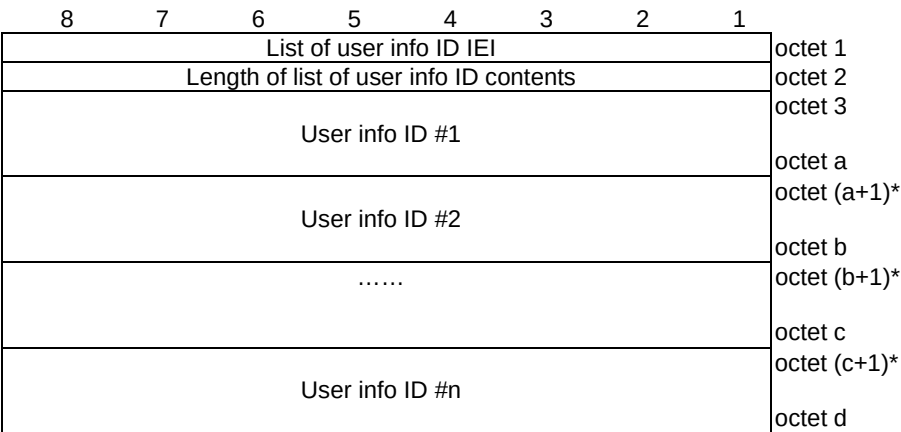
Figure 11.3.47.1: List of user info ID information element
