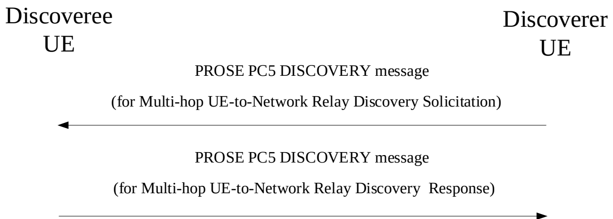
Figure 8b.2.1.3.3.2.1: Discoveree UE procedure for intermediate UE-to-network Relay discovery
