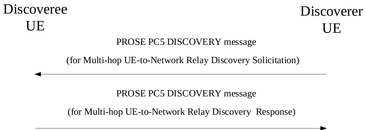
Figure 8b.2.1.3.3.2.1: Discoveree intermediate UE procedure for multi-hop UE-to-network relay discovery
