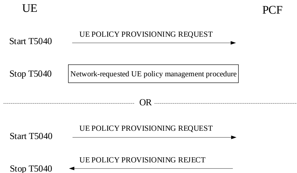
Figure 5.3.2.2.1: UE-requested ProSeP policy provisioning procedure
