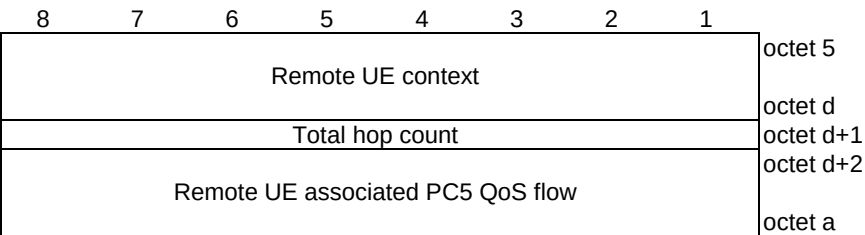
Figure 11.3.58.2: Remote UE parameters
