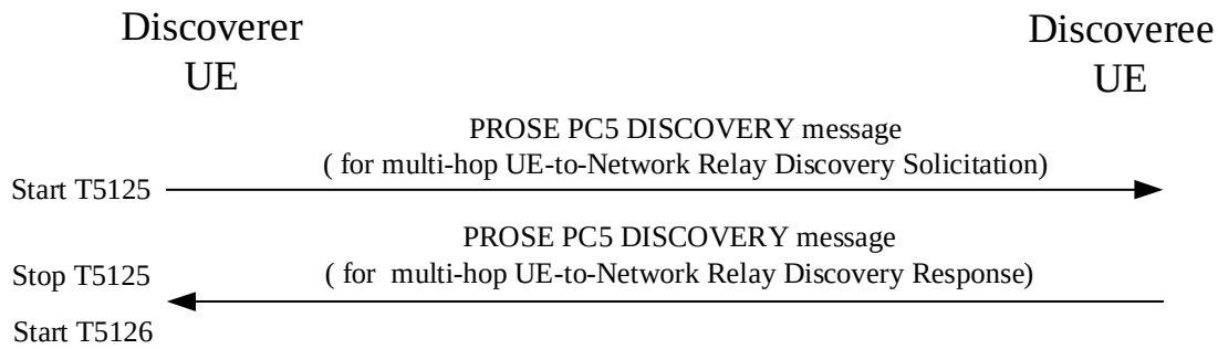
Figure 8b.2.1.3.2.3.1: Discoverer intermediate UE procedure for multi-hop UE-to-network Relay discovery
