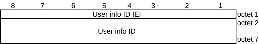
Figure 11.2.7.1: User info ID information element
