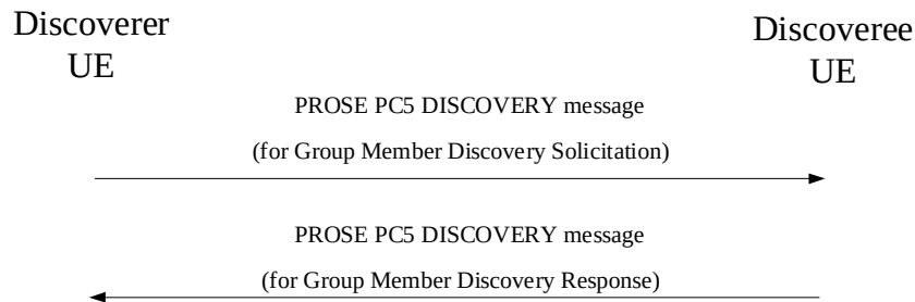
Figure 6.2.15.2.2.2.1: Discoverer UE procedure for group member discovery
