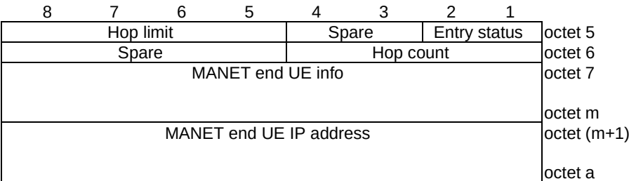
Figure 11.8.1.3: MANET discovery entry
