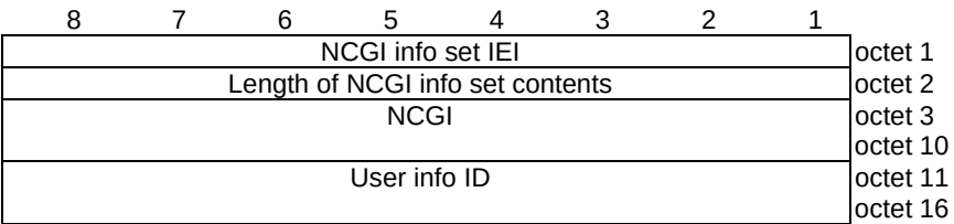
Figure 11.2.25.1: NCGI info set information element
