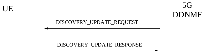
Figure 6.2.12.3.1.1: New ProSe restricted code allocation procedure
