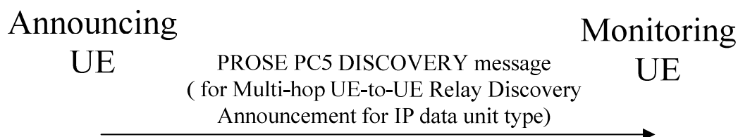
Figure 8c.2.1.2.2.3.2.1: Monitoring UE procedure for multi-hop layer-3 UE-to-UE relay discovery for IP data unit type
