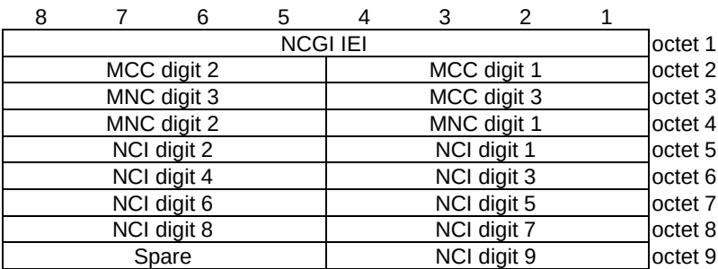
Figure 11.2.12.1: UE-to-network relay NCGI parameter
