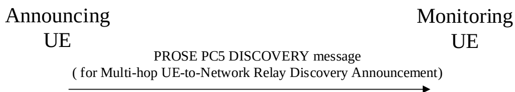
Figure 8b.2.1.2.3.2-1: ProSe intermediate UE-to-network relay UE procedure for multi-hop UE-to-network relay discovery monitoring
