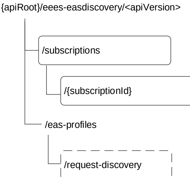
Figure 6.3.2.1-1: Resource URI structure of the Eees_EASDiscovery API
