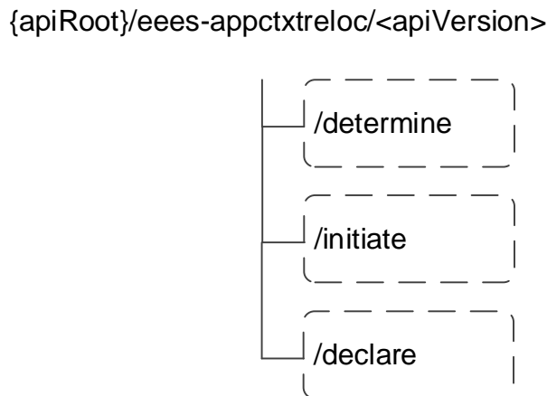
Figure 6.5.3.1-1: Resource URI structure of the Eees_AppContextRelocation API
