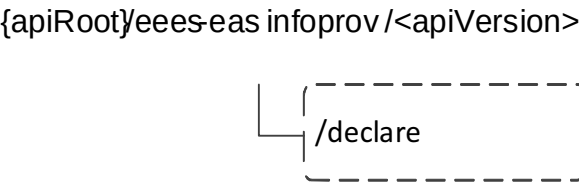
Figure 6.6.3.1-1: Resource URI structure of the Eees_EASInformationProvisioning API
