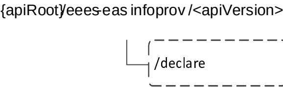
Figure 6.6.3.1-1: Resource URI structure of the Eees_EASInformationProvisioning API
