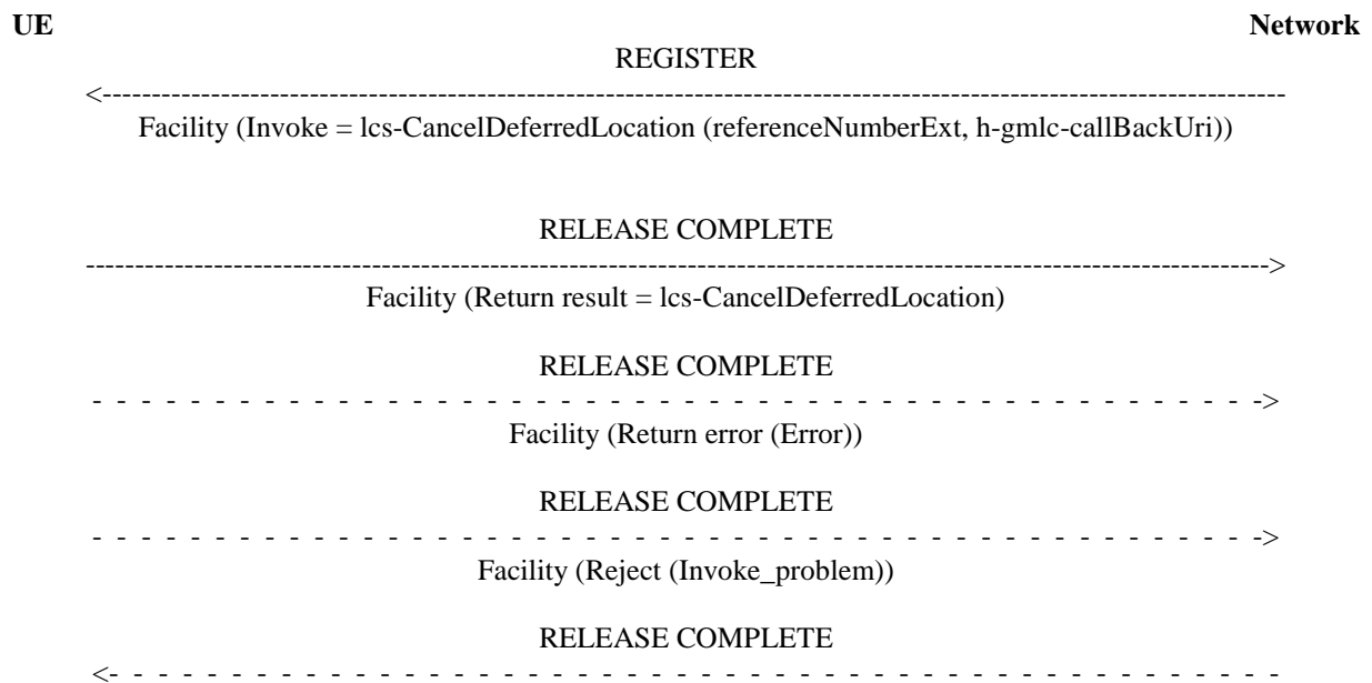
Figure 5.2.1.4.2.1: Cancel Deferred Location
