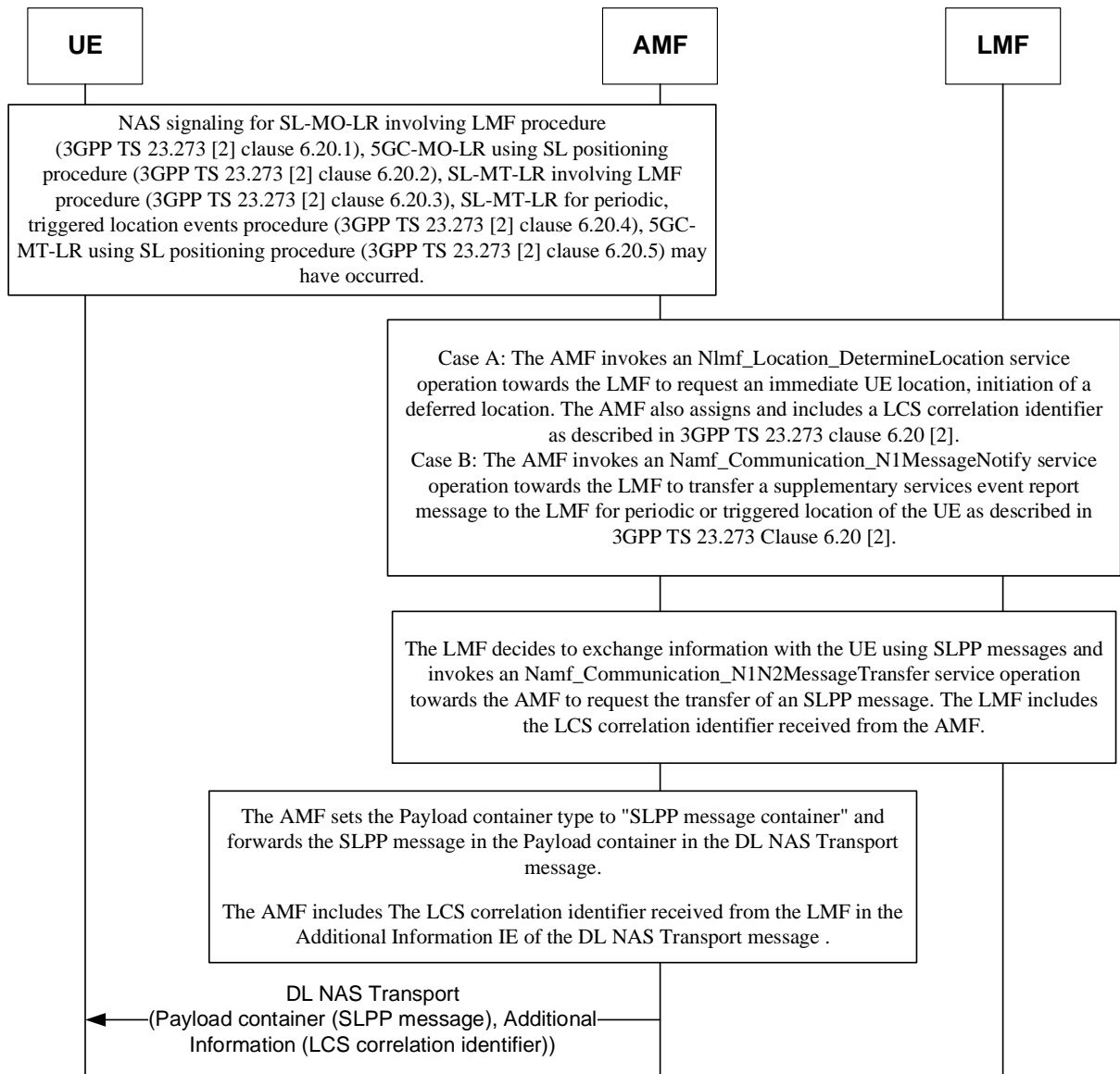
Figure 5.2.1.6.1: NAS signalling transport for downlink SLPP messages
