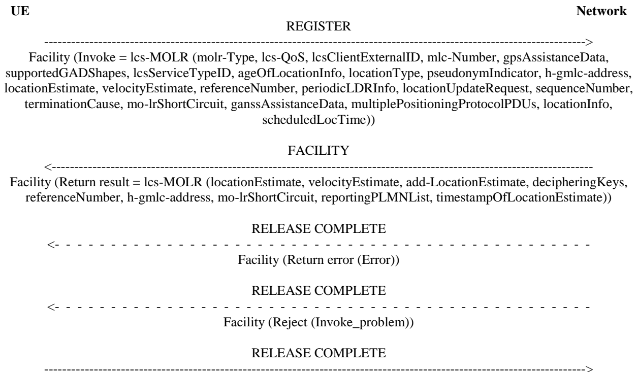
Figure 5.2.2.1.2-1: Single mobile originated location request
