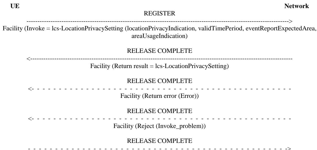
Figure 5.2.2.5.2-1: LocationPrivacySetting
