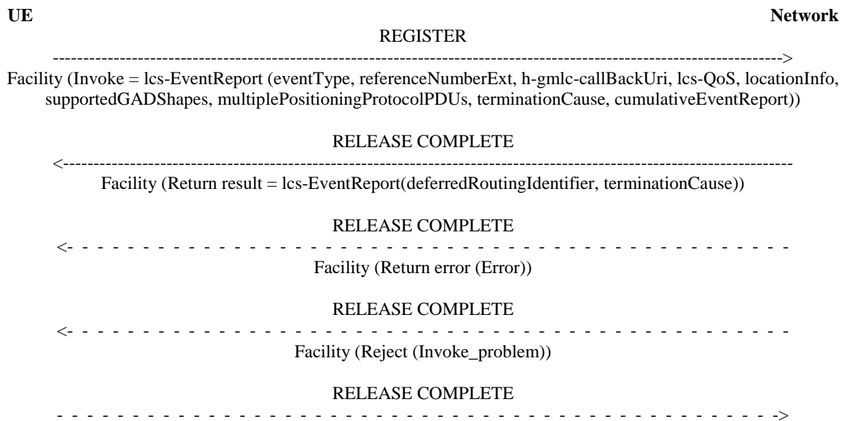
Figure 5.2.2.4.2-1: EventReport
