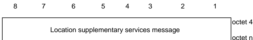
Figure 11.2.1.3: LCS-UP payload contents with LCS-UP payload type "Location supplementary services message"
