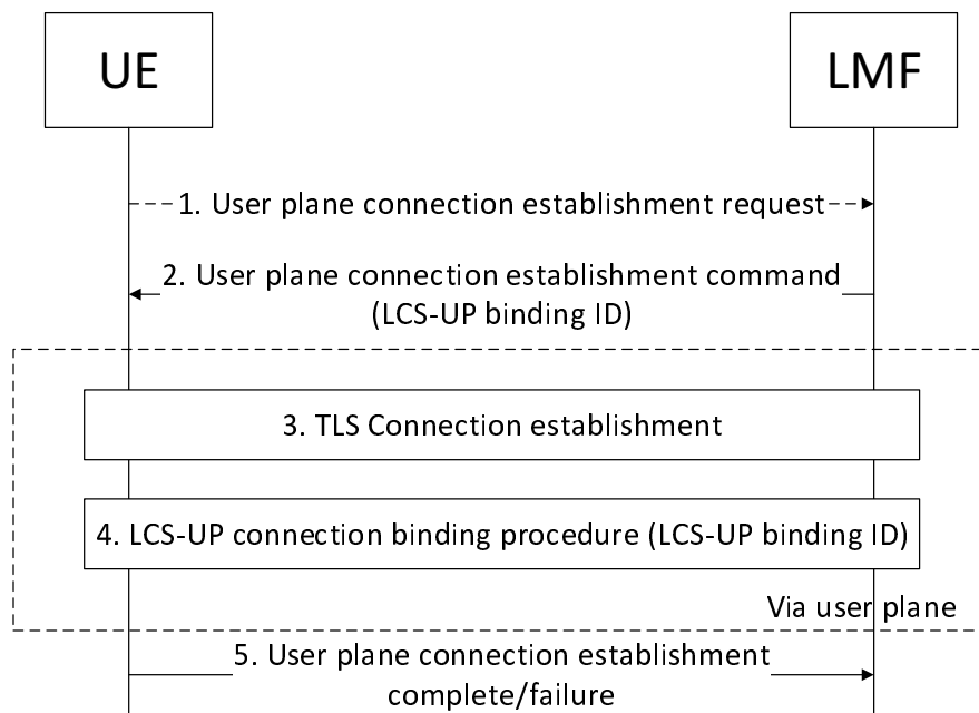
Figure A.1: Overall call flow for user plane connection establishment procedure with the LCS-UP connection binding procedure.
