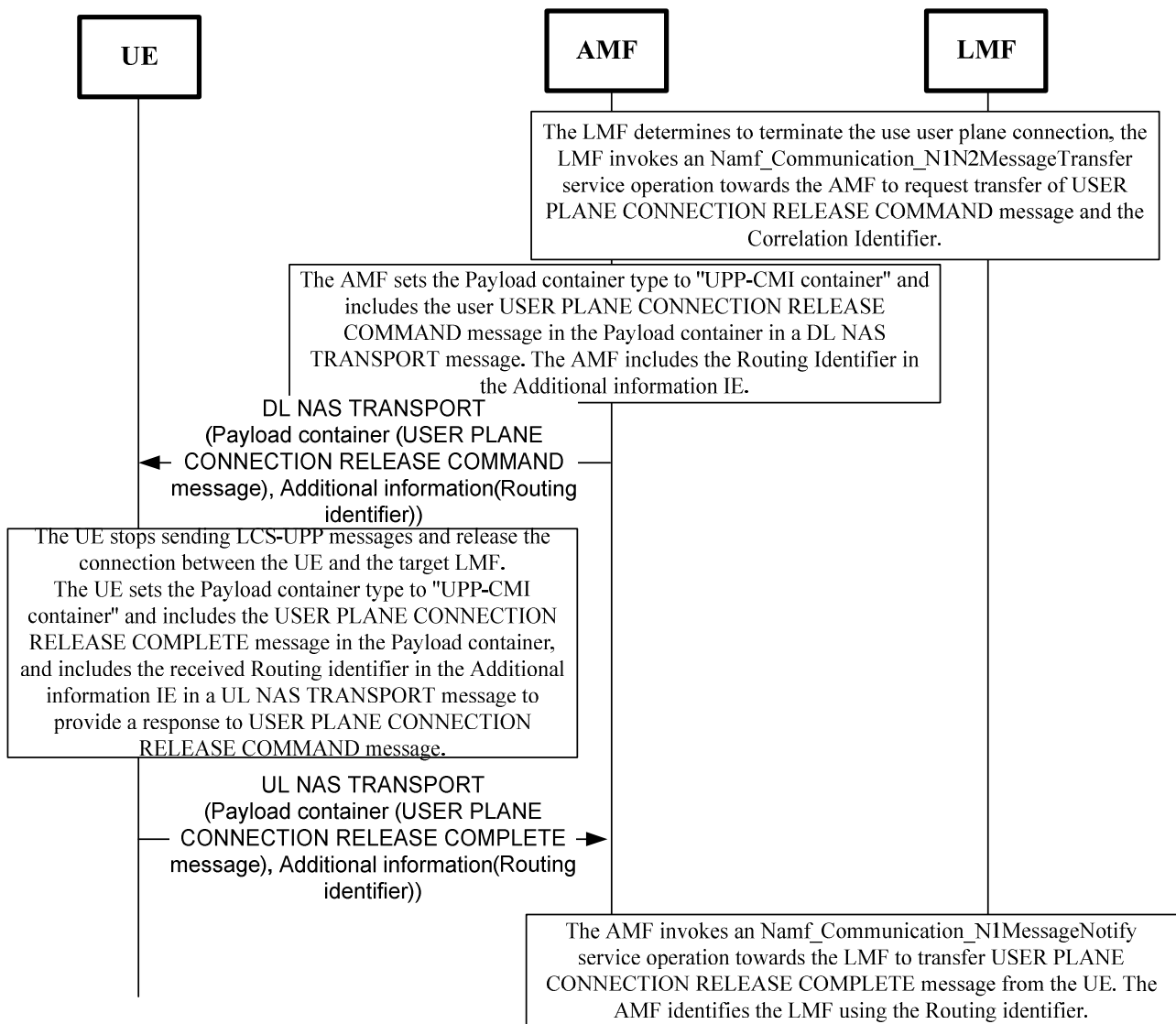
Figure 6.2.1.2.1.1: Signalling transport for network initiated user plane connection release procedure
