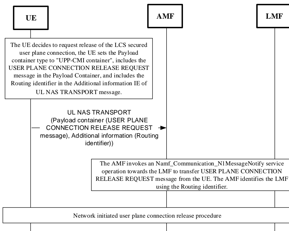
Figure 6.2.2.2.1.1: Signalling transport for UE requested user plane connection release procedure
