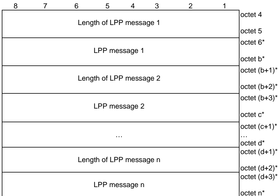
Figure 11.2.1.2: LCS-UP payload contents with LCS-UP payload type "LTE Positioning Protocol (LPP) message"
