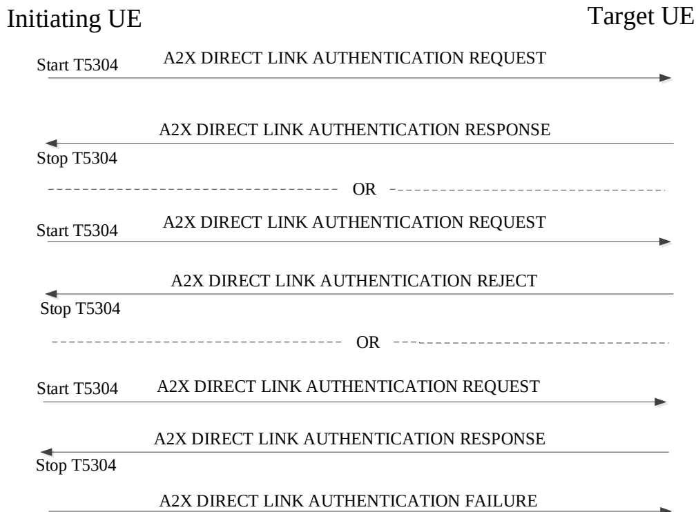
Figure 6.1.2.6.2: A2X PC5 unicast link authentication procedure
