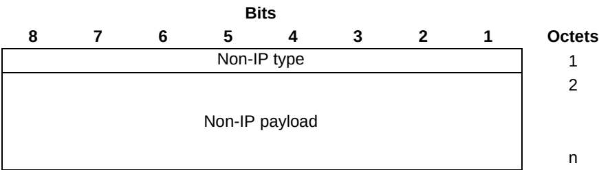
Figure 12A.3.1: Non-IP PDU format
