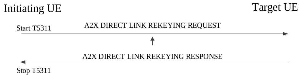
Figure 6.1.2.10.2: A2X PC5 unicast link re-keying procedure
