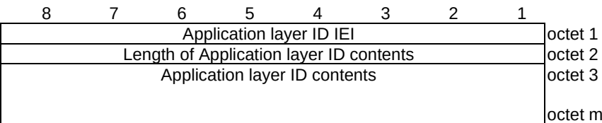
Figure 12.3.4.1: Application layer ID information element
