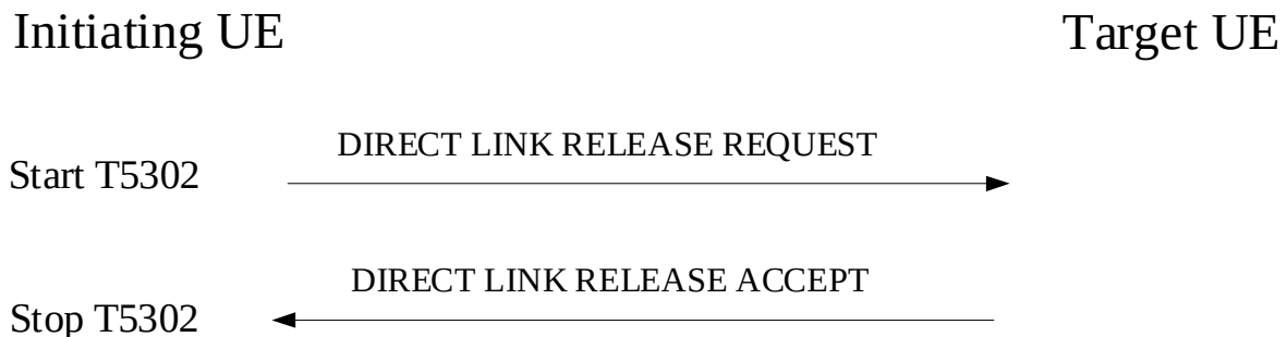
Figure 6.1.2.4.2.1: A2X PC5 unicast link release procedure
