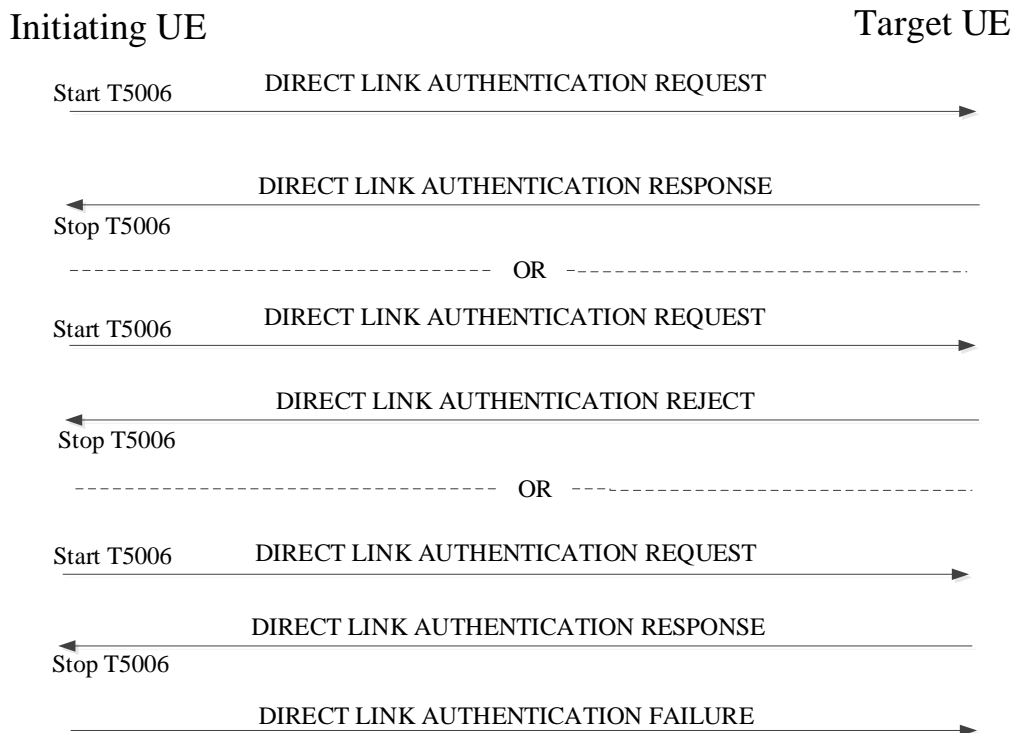
Figure 6.1.2.6.2: PC5 unicast link authentication procedure
