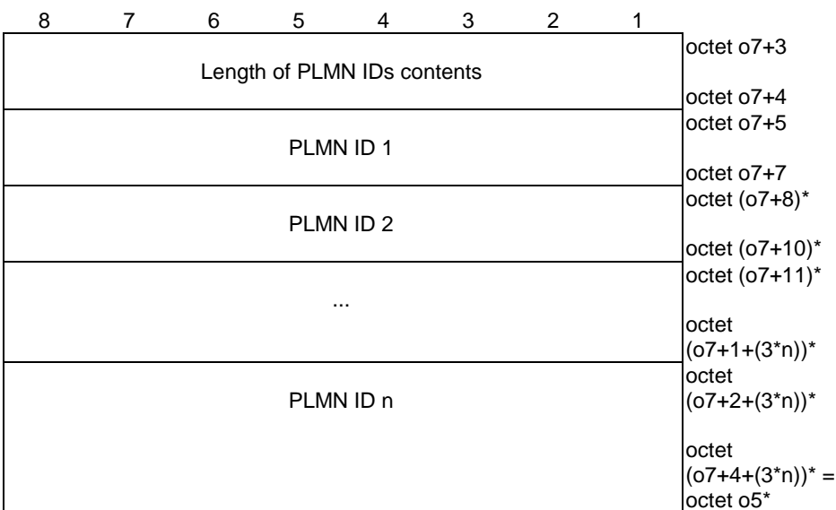
Figure 5.4.1.4: PLMN IDs
