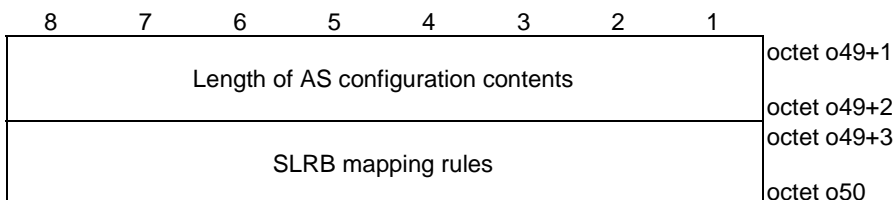
Figure 5.3.1.46a: AS configuration
