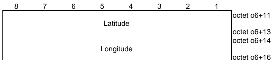
Figure 5.3.1.10: Coordinate area
