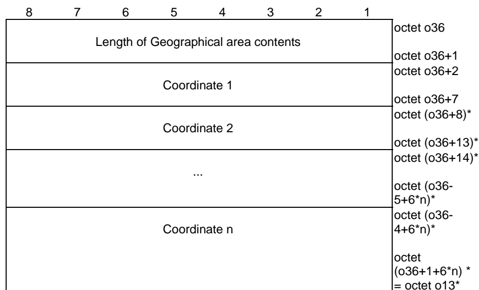
Figure 5.4.1.15: Geographical area
