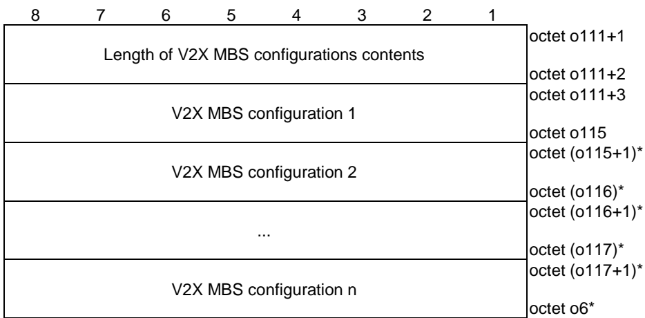
Figure 5.4.1.8A: V2X MBS configurations
