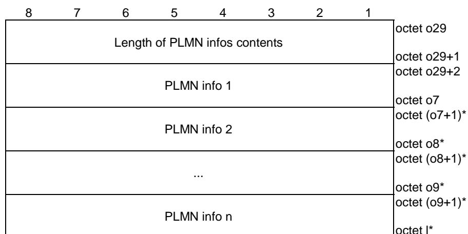
Figure 5.4.1.2: PLMN infos
