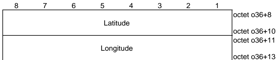
Figure 5.4.1.16: Coordinate area
