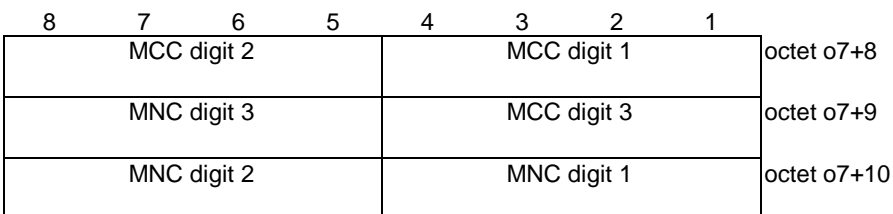
Figure 5.4.1.5: PLMN ID
