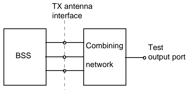
Figure 5.11.5.2: Transmitter test setup
