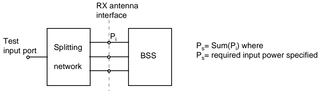
Figure 5.11.5.1: Receiver test setup
