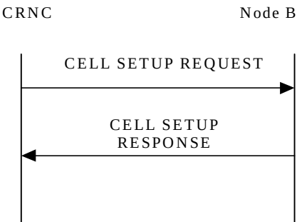
Figure 16: Cell Setup procedure, Successful Operation
