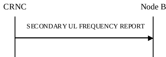
Figure 48A: Secondary UL Frequency Reporting procedure
