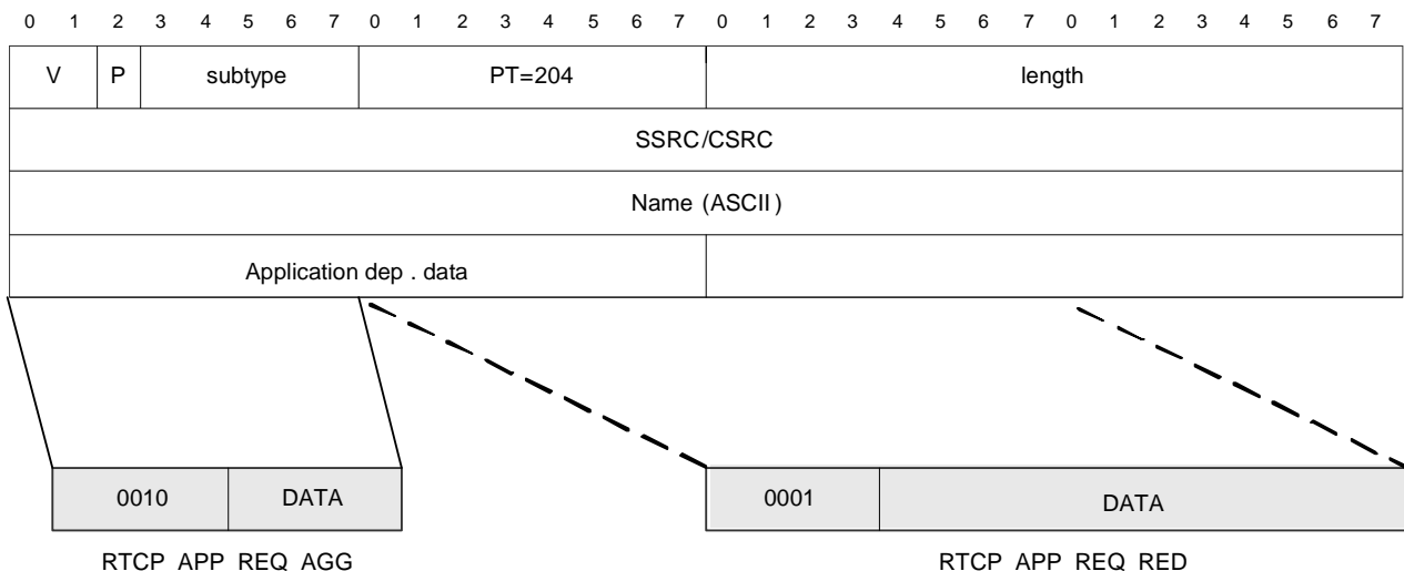
Figure 10.1: RTCP-APP formatting
