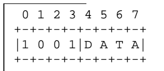
Figure 10.6g: IVAS Coded Format request
