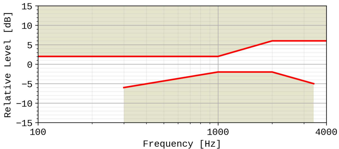
Figure 6b: Handset and headset receiving sensitivity/frequency mask
