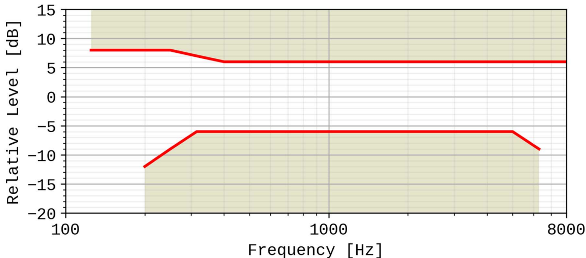
Figure 12: Desktop hands-free receiving sensitivity/frequency mask
