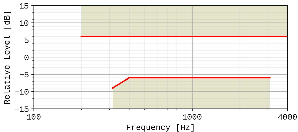
Figure 4: Desktop receiving sensitivity/frequency mask
