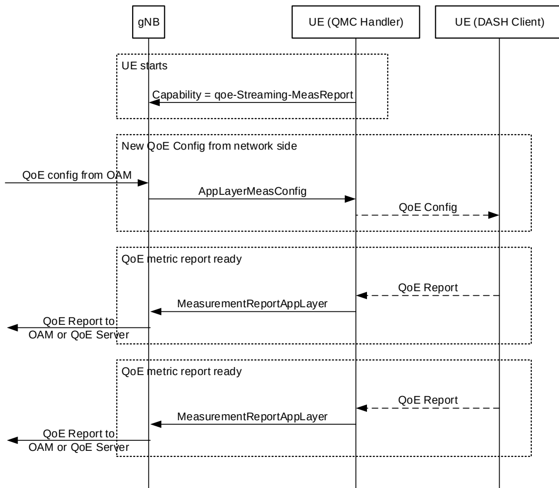
Figure L-3: Example signalling diagram for NR
