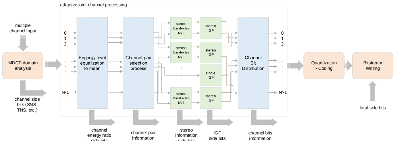
Figure 5.2-27: Block diagram of MCT and the adaptive joint channel processing
