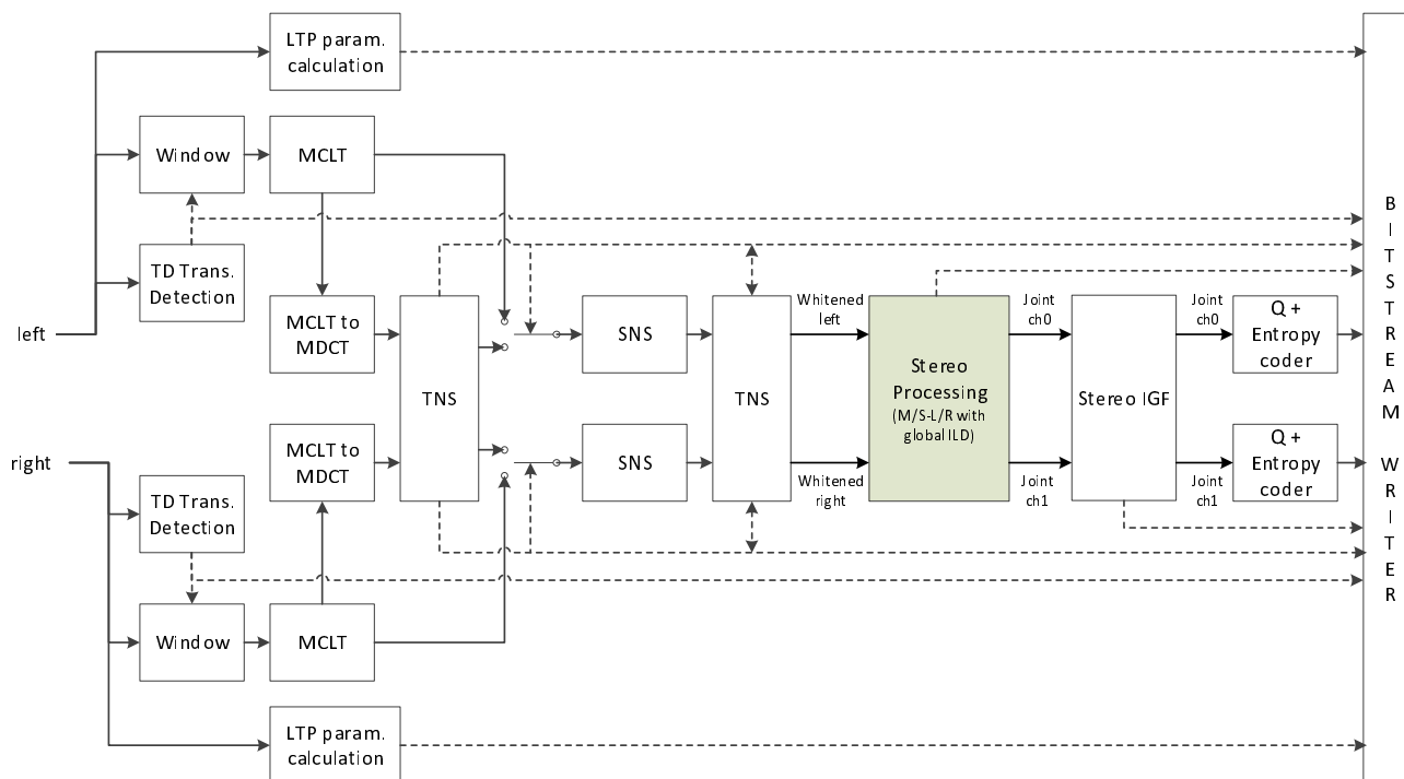
Figure 5.3-37: Block diagram of the MDCT-based stereo encoder
