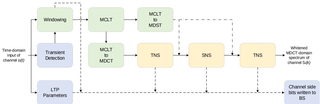
Figure 5.2-26: Block diagram of whitening preprocessing for each channel
