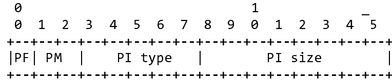
Figure A.3.5.2-1: PI data header.
