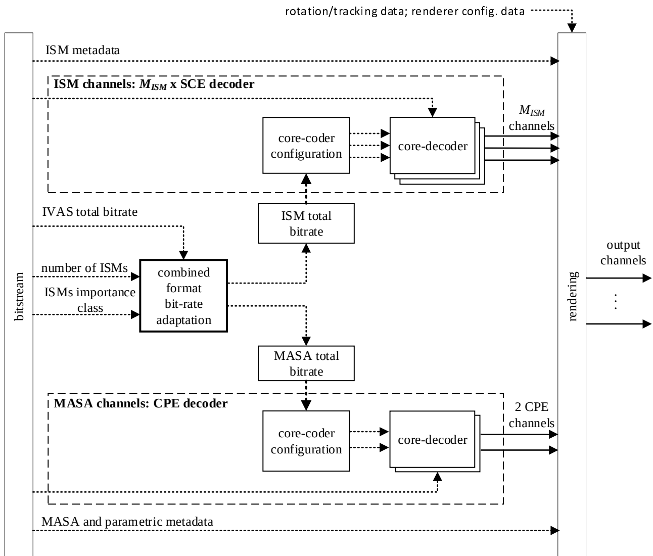
Figure 6.9-1: Block diagram of OMASA decoder
