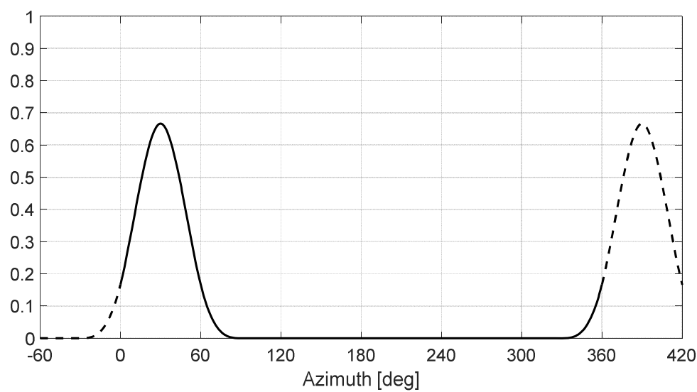
Figure 7.2-3: Example of periodic azimuth basis function.
