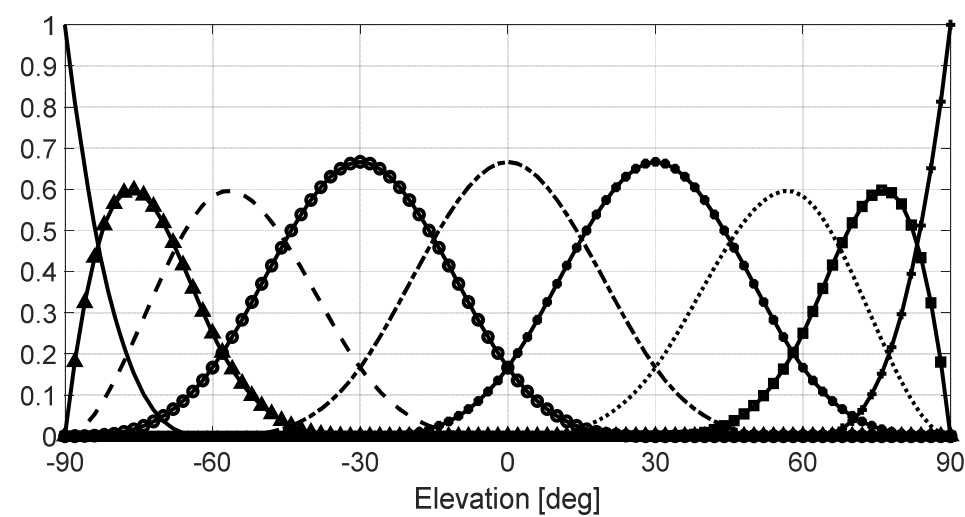
Figure 7.2-4: Example of standard B-spline basis functions for elevation.
