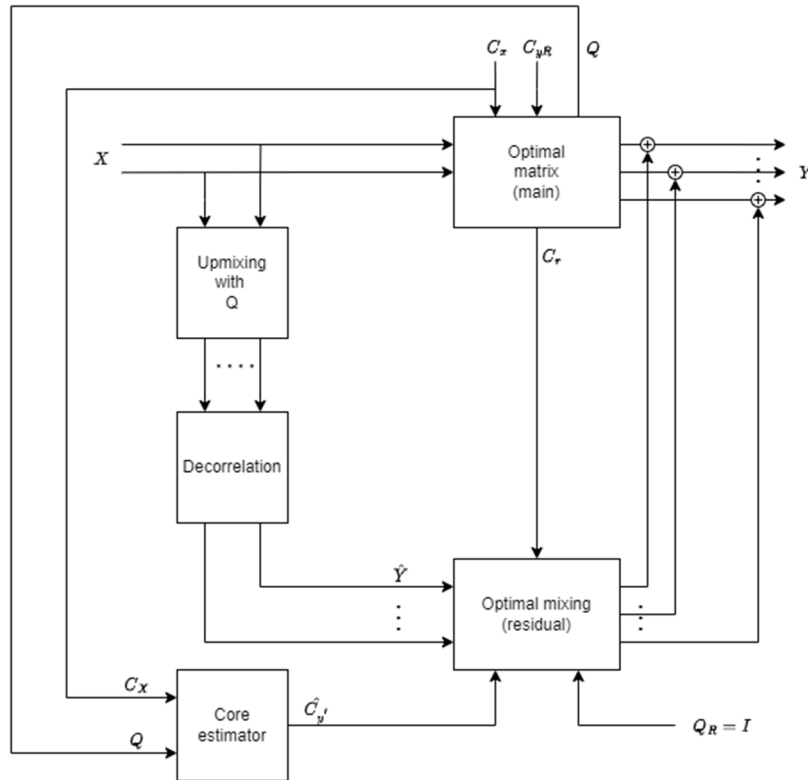
Figure 6.7-2: ParamMC Synthesis
