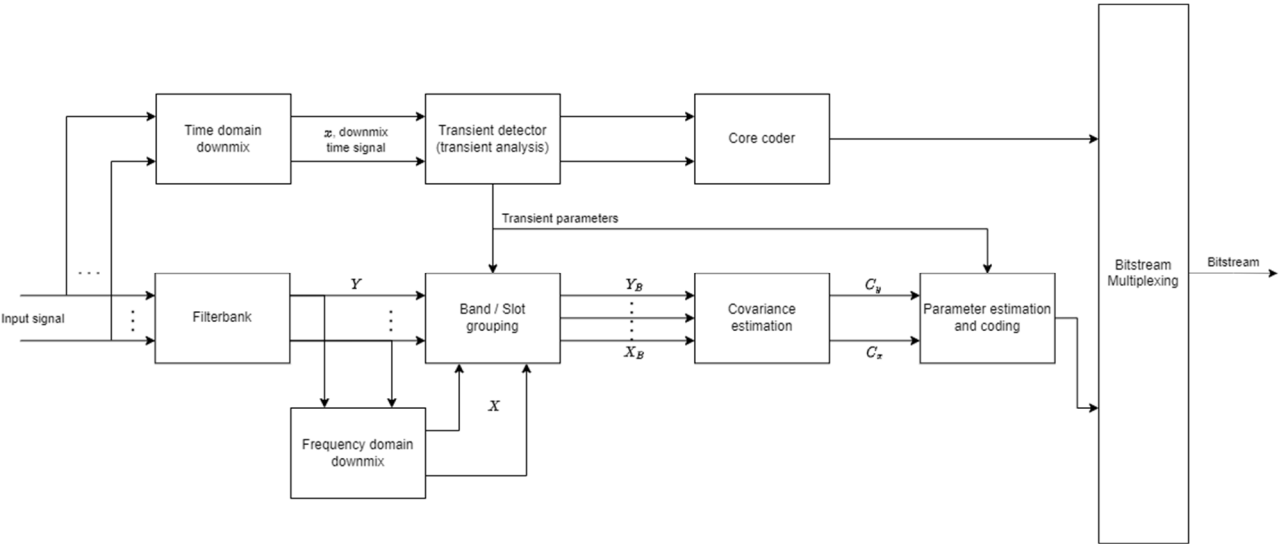
Figure 5.7-3: ParamMC Encoder
