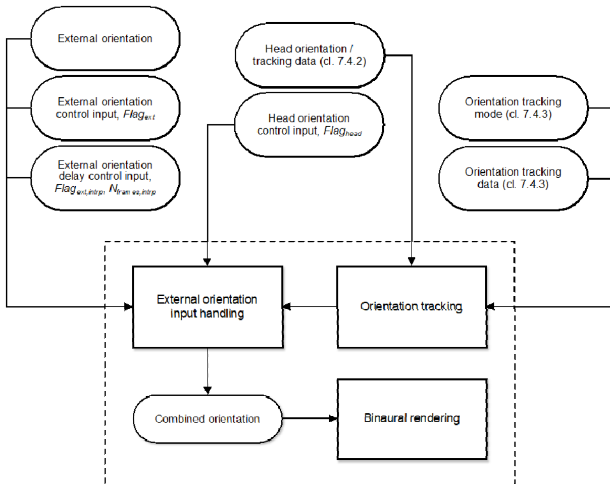
Figure 7.4-4: Block diagram of external orientation input handling for binaural rendering
