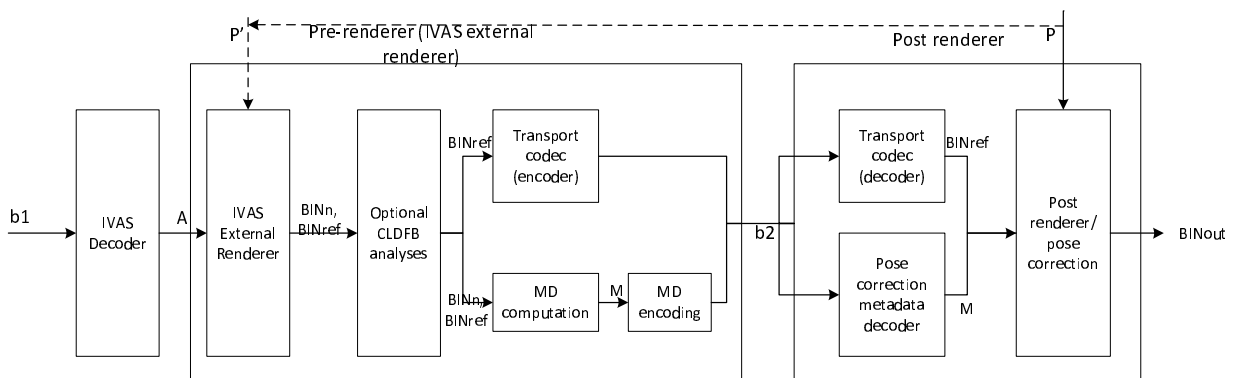
Figure 7.6-2: Split rendering architecture with IVAS external renderer
