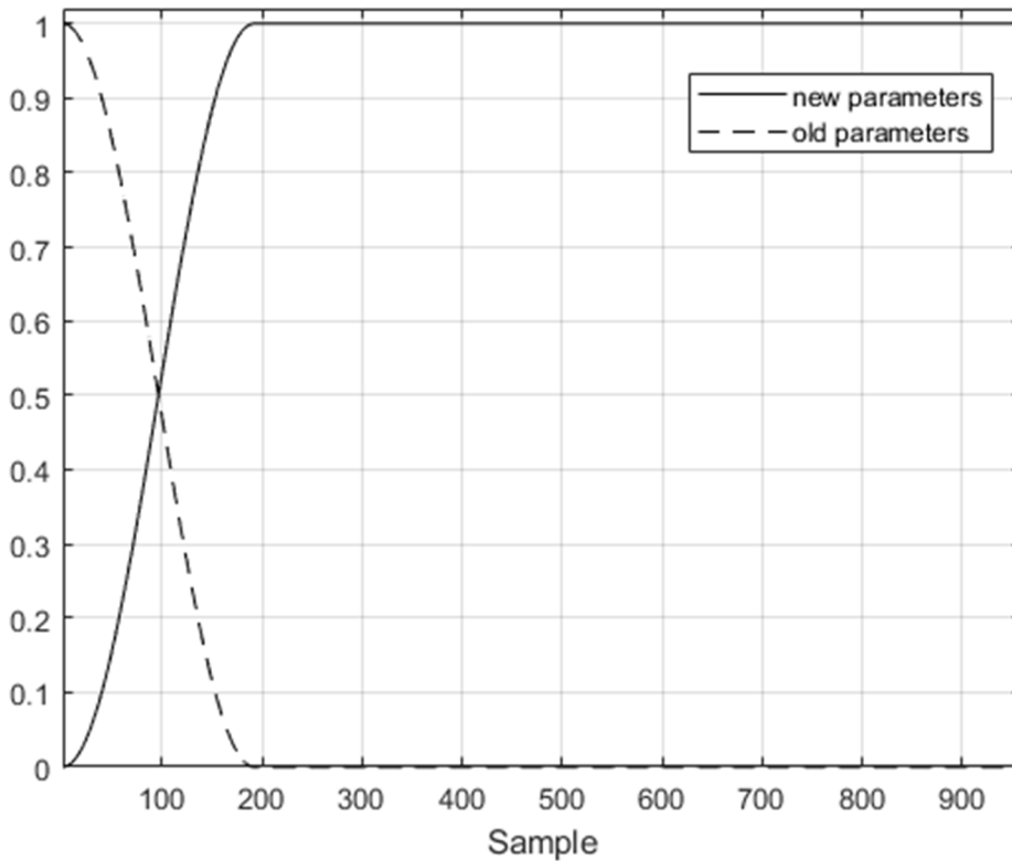
Figure 5.4-11: Cross-fading windows
