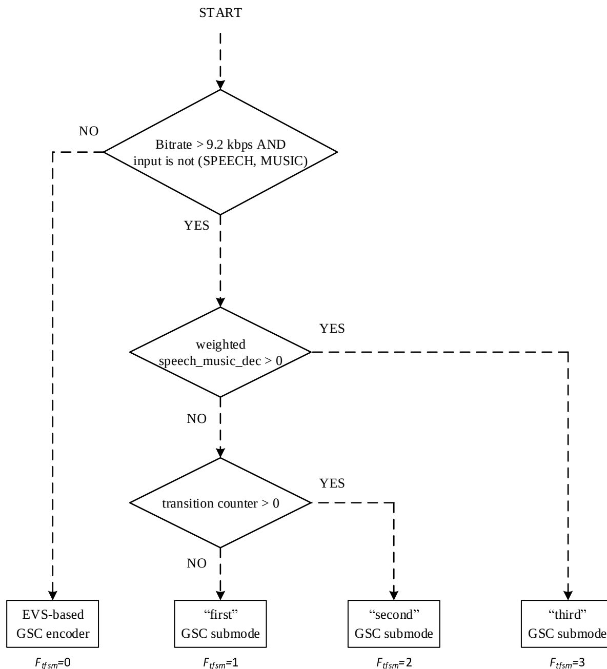
Figure 5.2-14: GSC sub-mode selection
