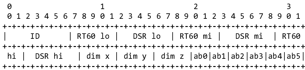
Figure A.3.5.6.2-3: Acoustic environment PI data frame (ACOUSTIC_ENVIRONMENT) containing a compact AE representation with late reverb and early reflection parameters.
