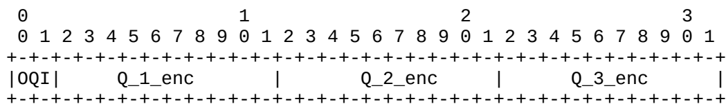
Figure A.3.5.6.1.1-1: PI orientation data as quaternions.
