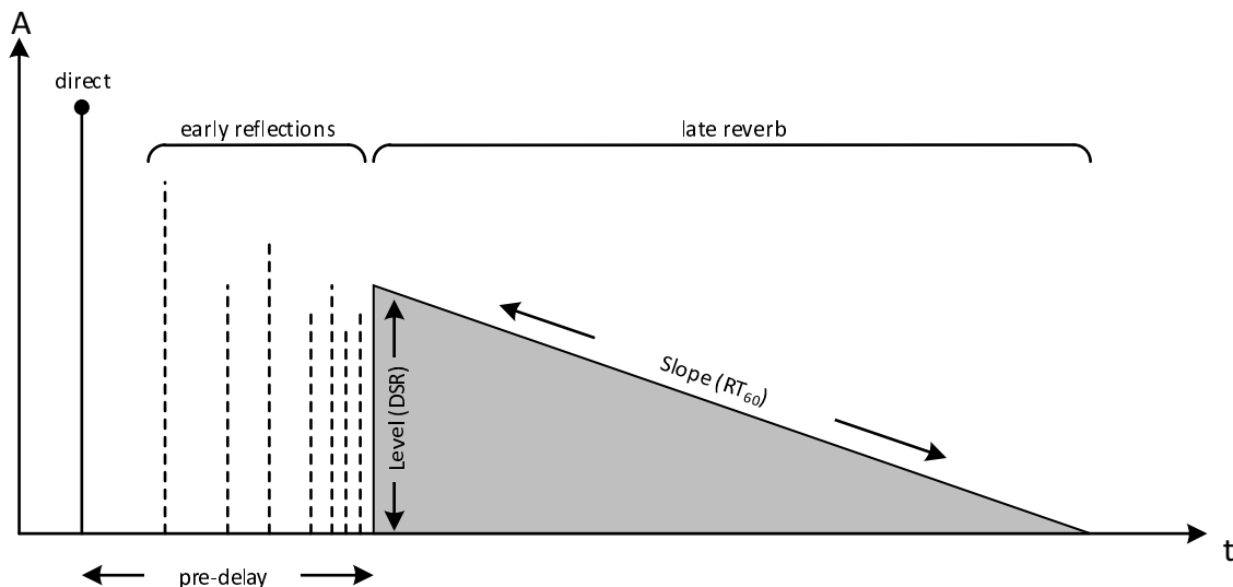
Figure 7.4-9: Simple representation of the main reverberation properties
