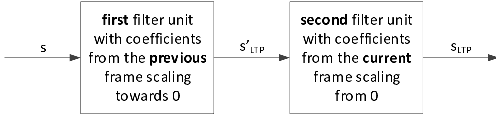
Figure 6.2-12: Block diagram of the LTP post filtering
