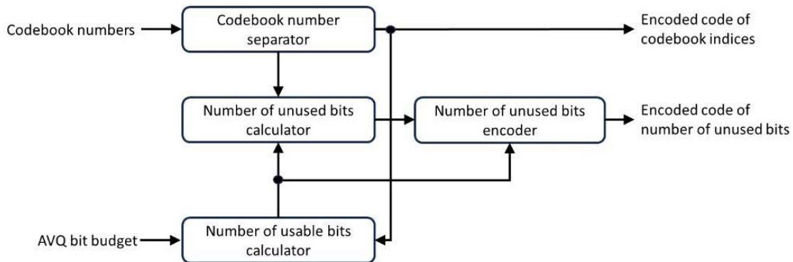
Figure 5.2-8: Functional Block Diagram of Code Converter
