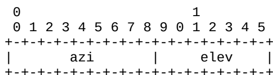
Figure A.3.5.7.7.8-1: R_ISM_DIRECTION PI data frame.
