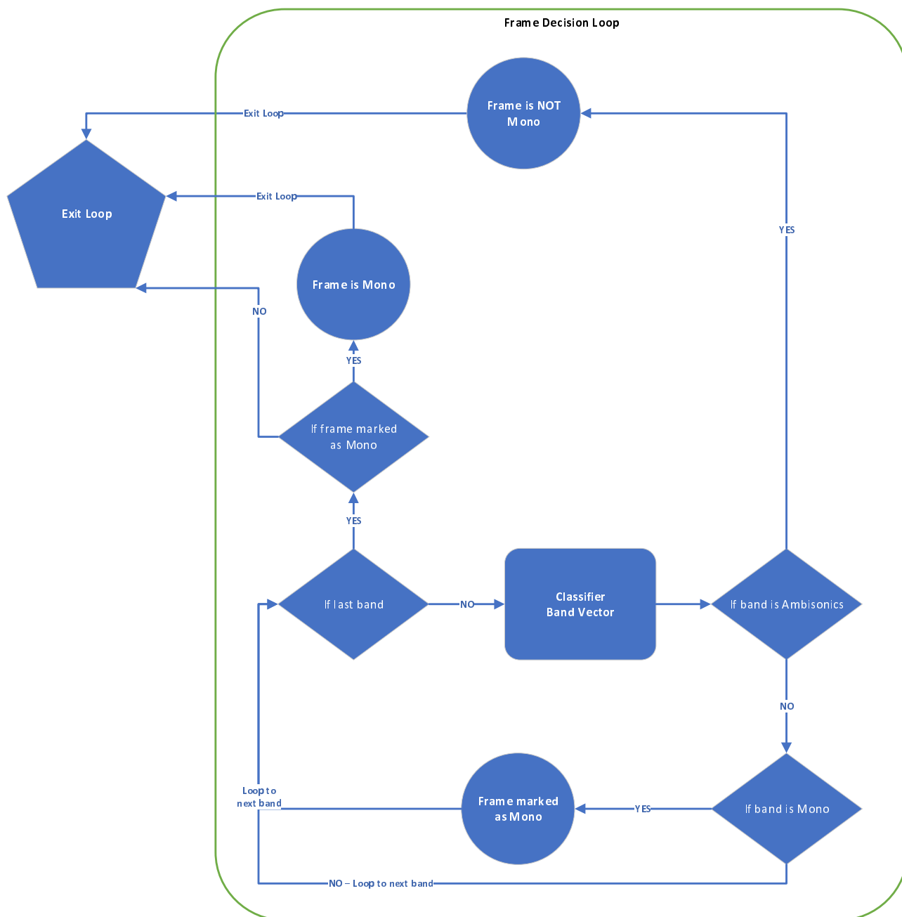
Figure 5.4-10: Mono Detector Frame Decision Loop
