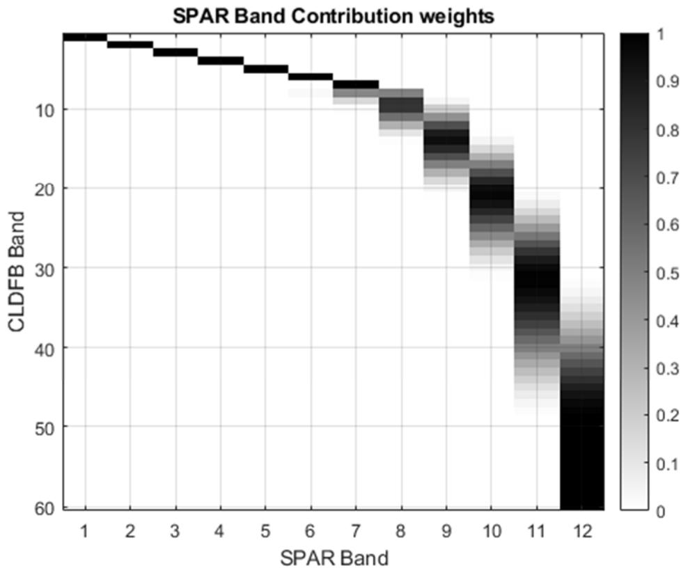
Figure 6.4-7: SPAR Band contributions H_l^b
