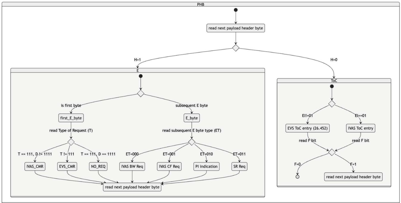
Figure A.3.3.3.4-1: State Machine for parsing a Payload Header Byte.
