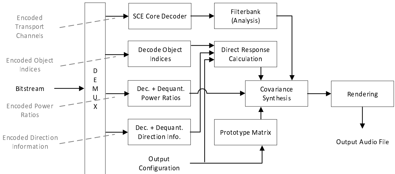
Figure 6.6-2: ParamISM decoder overview
