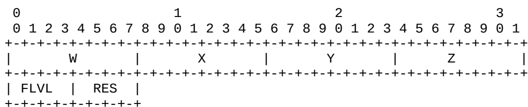
Figure A.3.5.7.5.1-1: Audio focus PI data frame with direction and level.
