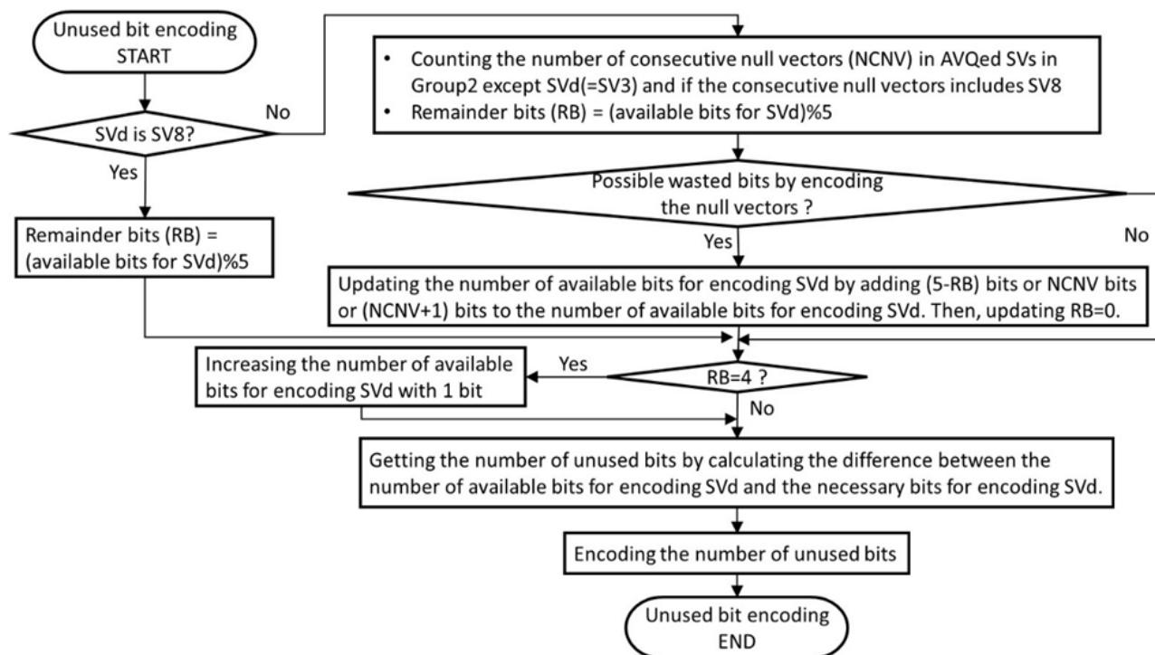
Figure 5.2-12: Flow of Encoding the number of unused bits
