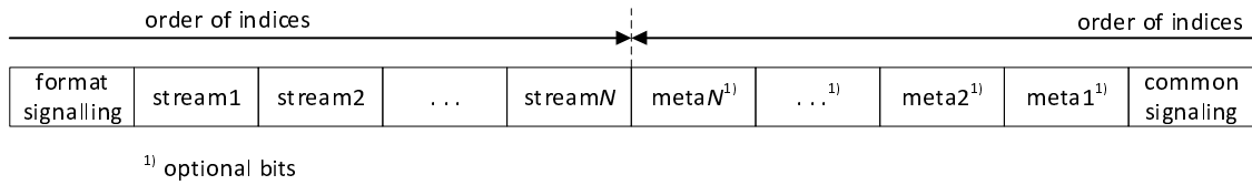
Figure 5.6-4: Structure of ISM format bitstream
