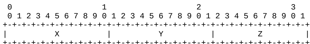
Figure A.3.5.6.4.6-1: Compact position PI data frame with cartesian coordinates.
