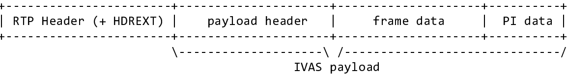
Figure A.3.3.2-1: RTP Header with IVAS payload structure
