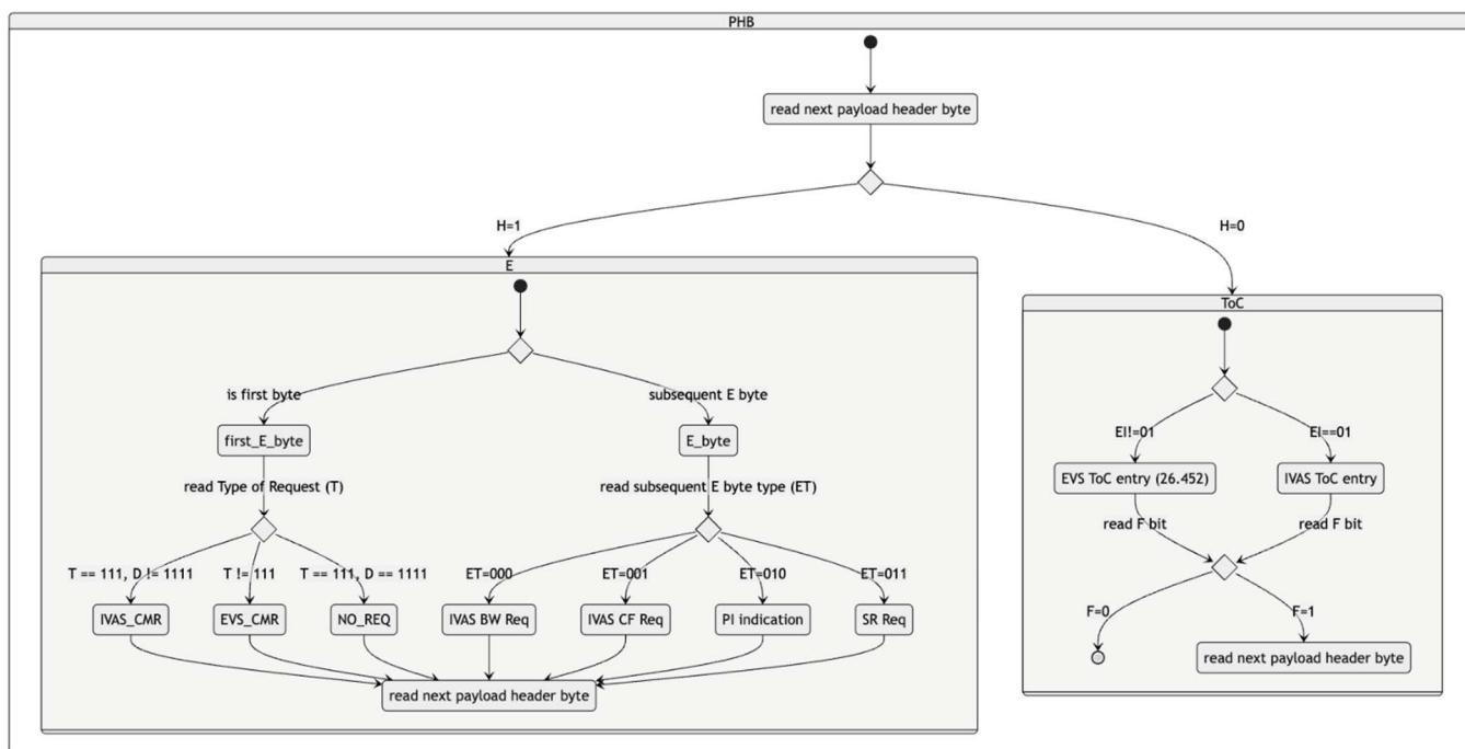
Figure A.3.3.3.4-1: State Machine for parsing a Payload Header Byte.
