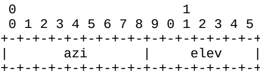
Figure A.3.5.7.7.8-1: R_ISM_DIRECTION PI data frame.
