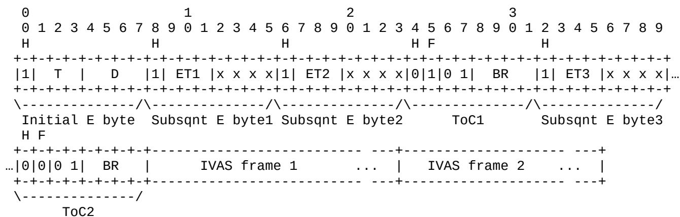
Figure A.3.3.3.4-2: Payload structure with IVAS frames and E bytes in the payload.
