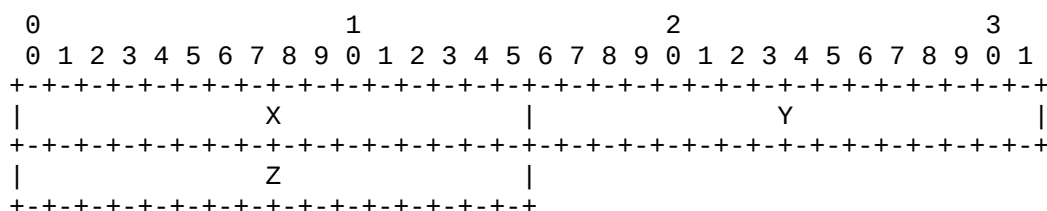
Figure A.3.5.7.3-1: General position PI data frame with cartesian coordinates.
