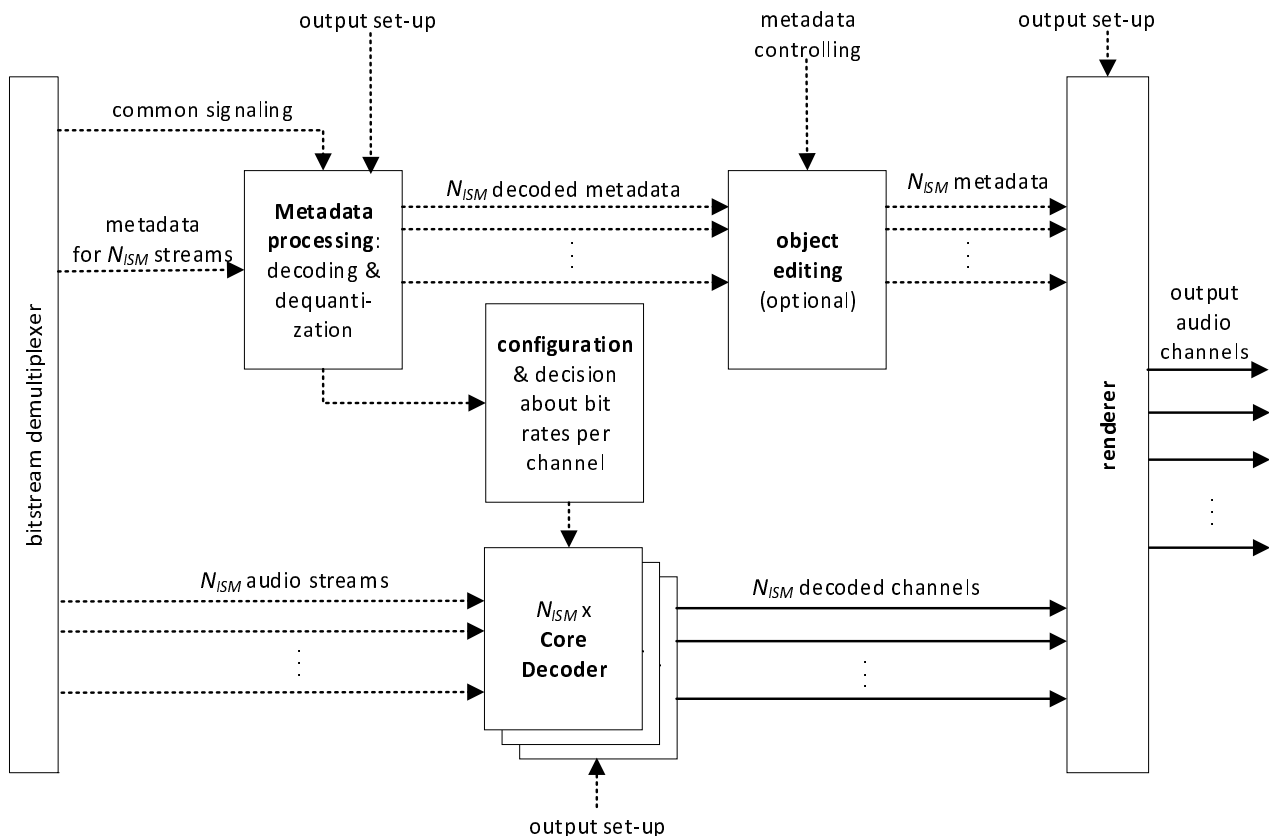
Figure 6.6-1: Block diagram of the DiscISM decoder
