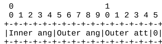
Figure A.3.5.6.4.8-1: ISM_DIRECTIVITY PI data frame.
