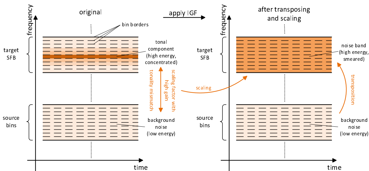
Figure 5.2-21: Illustration of noise bands due to tonality mismatch
