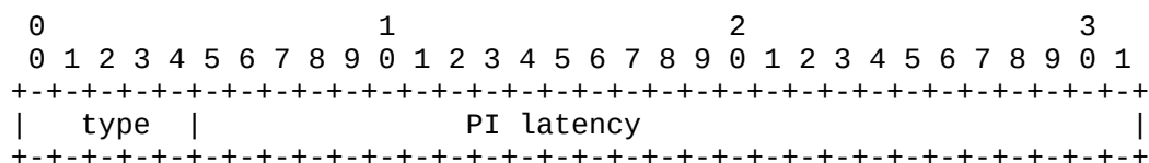
Figure A.3.5.7.6-1: PI latency indication.
