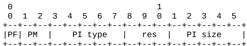
Figure A.3.5.2-1: PI data header.
