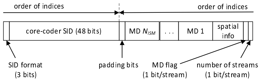
Figure 5.6-6: Structure of SID ISM format bitstream
