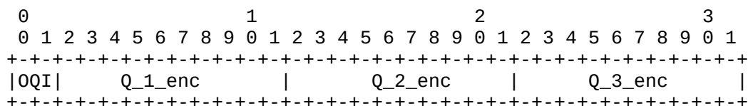
Figure A.3.5.6.1.1-1: PI orientation data as quaternions.
