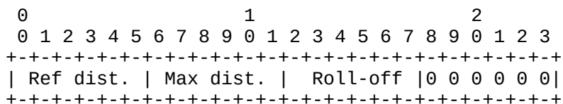
Figure A.3.5.6.4.7-1: ISM_DISTANCE_ATTENUATION PI data frame.
