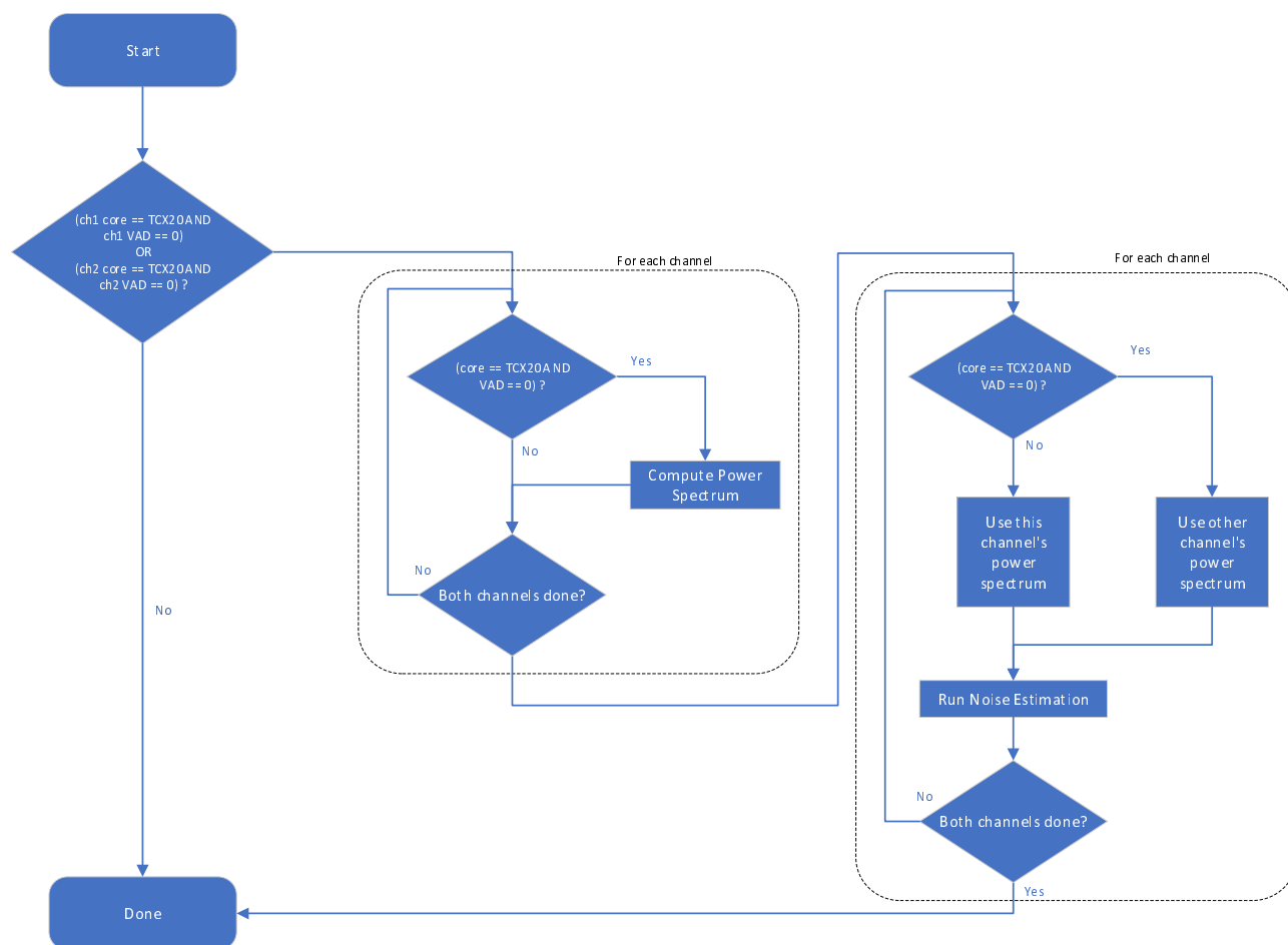
Figure 6.3-11: Background noise estimation in MDCT Stereo
