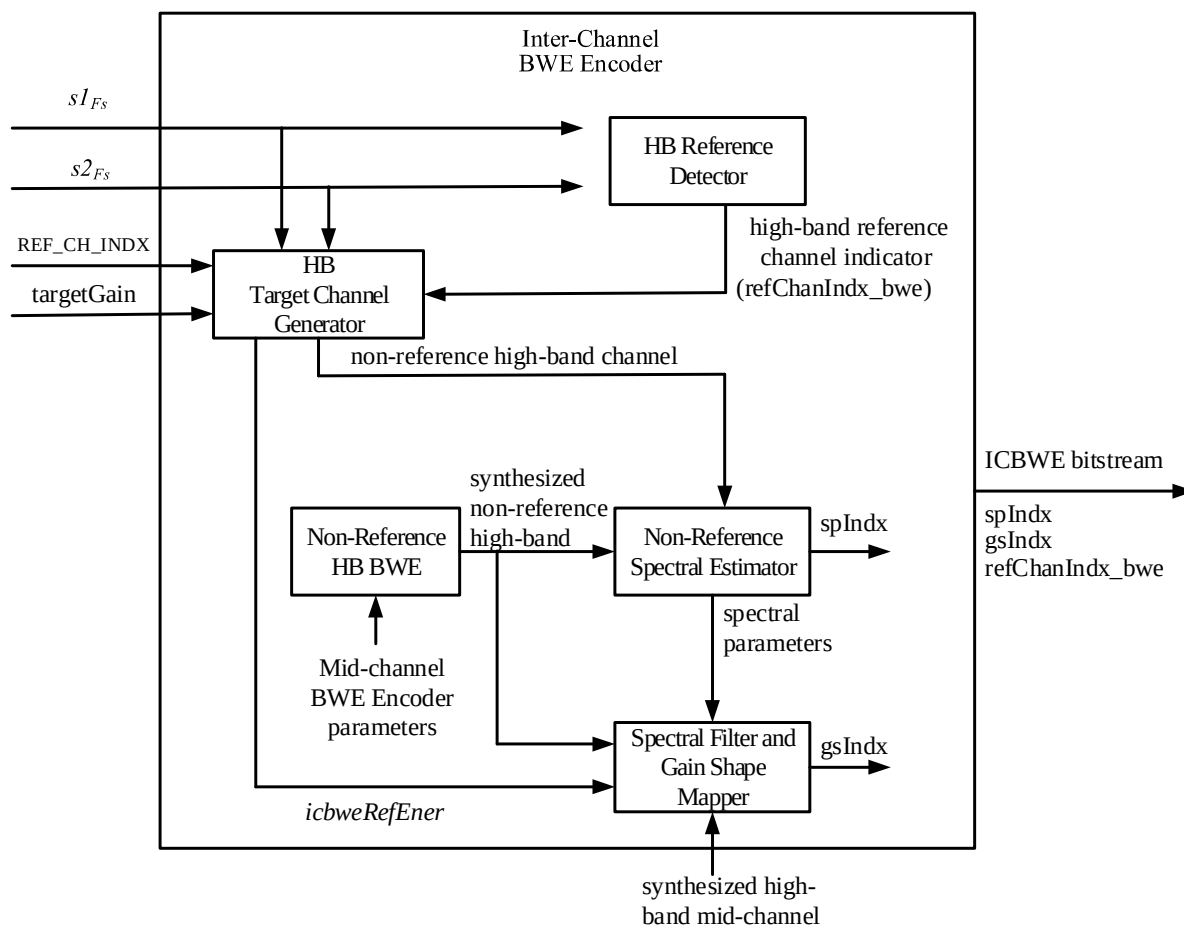
Figure 5.3-4: Block diagram of the IC-BWE Encoder
